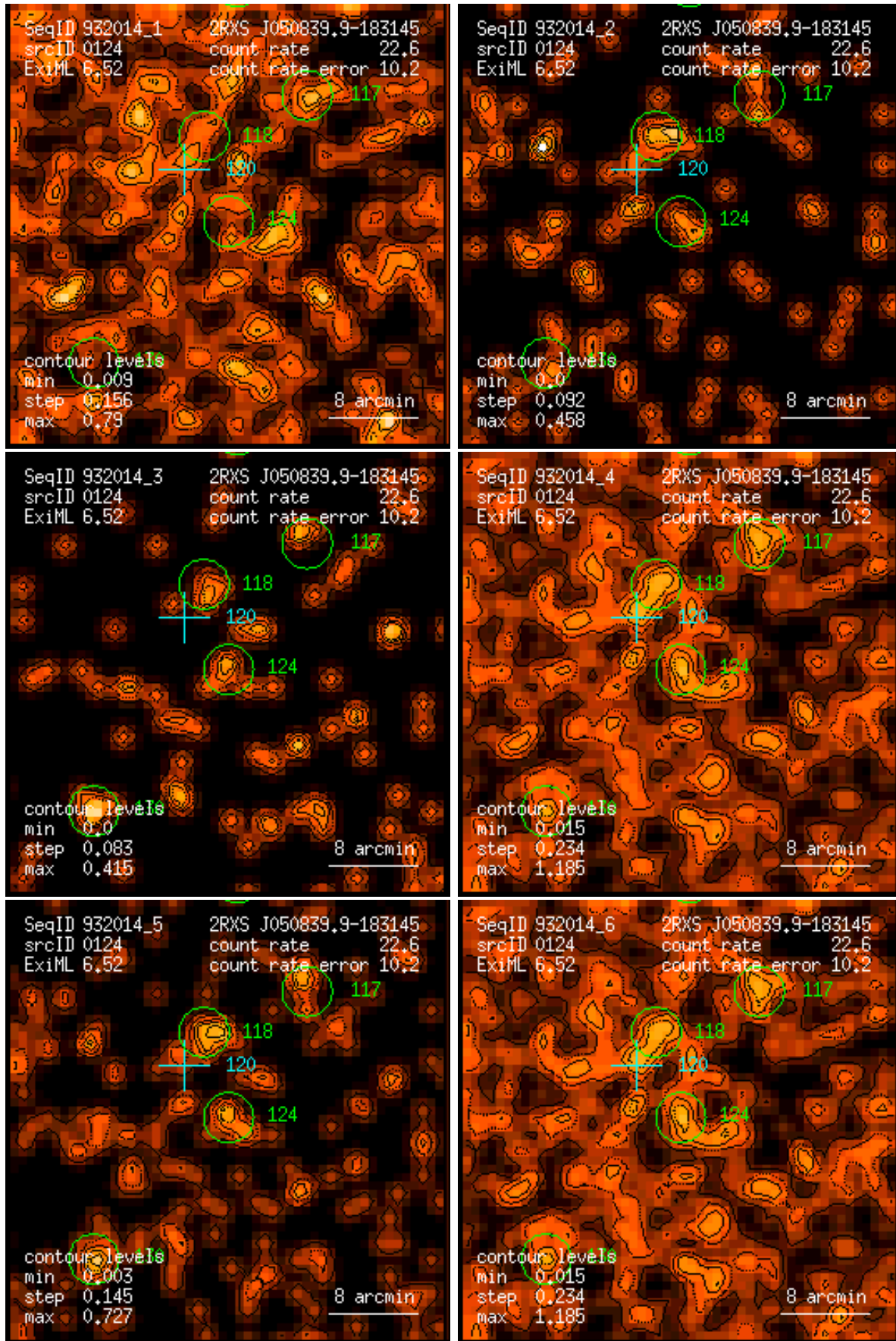
Figure 124: RASS 932014: detection 0124: band rate images, Gaussian filter: (1) PSPC channels 11 – 41, (2) 52 – 90, (3) 91 – 201, (4) 11 – 235, (5) 52 – 201, (6) 11 – 201. Broad band rates in counts/ks. Band rate contour levels in counts/ks/arcmin 2 .
