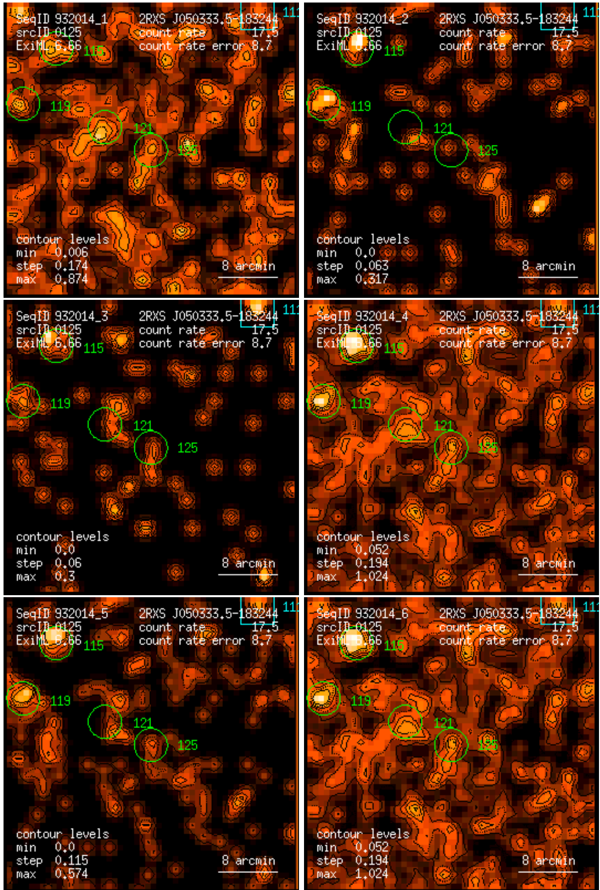
Figure 125: RASS 932014: detection 0125: band rate images, Gaussian filter: (1) PSPC channels 11 – 41, (2) 52 – 90, (3) 91 – 201, (4) 11 – 235, (5) 52 – 201, (6) 11 – 201. Broad band rates in counts/ks. Band rate contour levels in counts/ks/arcmin 2 .
