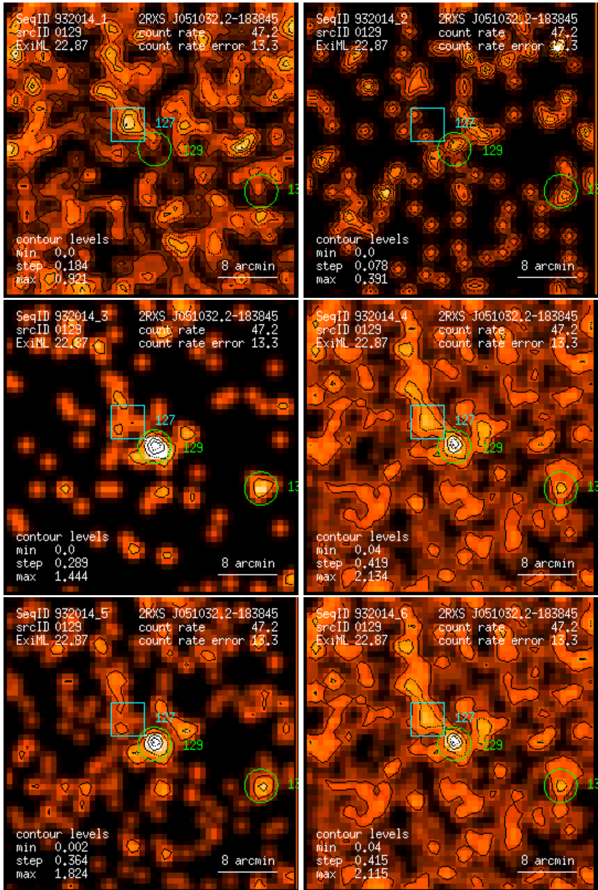
Figure 129: RASS 932014: detection 0129: band rate images, Gaussian filter: (1) PSPC channels 11 – 41, (2) 52 – 90, (3) 91 – 201, (4) 11 – 235, (5) 52 – 201, (6) 11 – 201. Broad band rates in counts/ks. Band rate contour levels in counts/ks/arcmin 2 .
