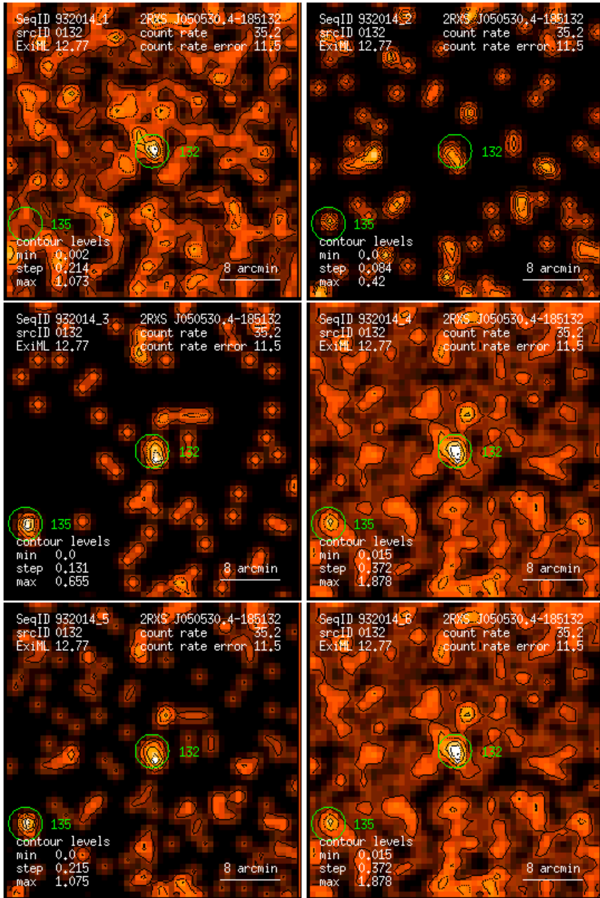
Figure 132: RASS 932014: detection 0132: band rate images, Gaussian filter: (1) PSPC channels 11 – 41, (2) 52 – 90, (3) 91 – 201, (4) 11 – 235, (5) 52 – 201, (6) 11 – 201. Broad band rates in counts/ks. Band rate contour levels in counts/ks/arcmin 2 .
