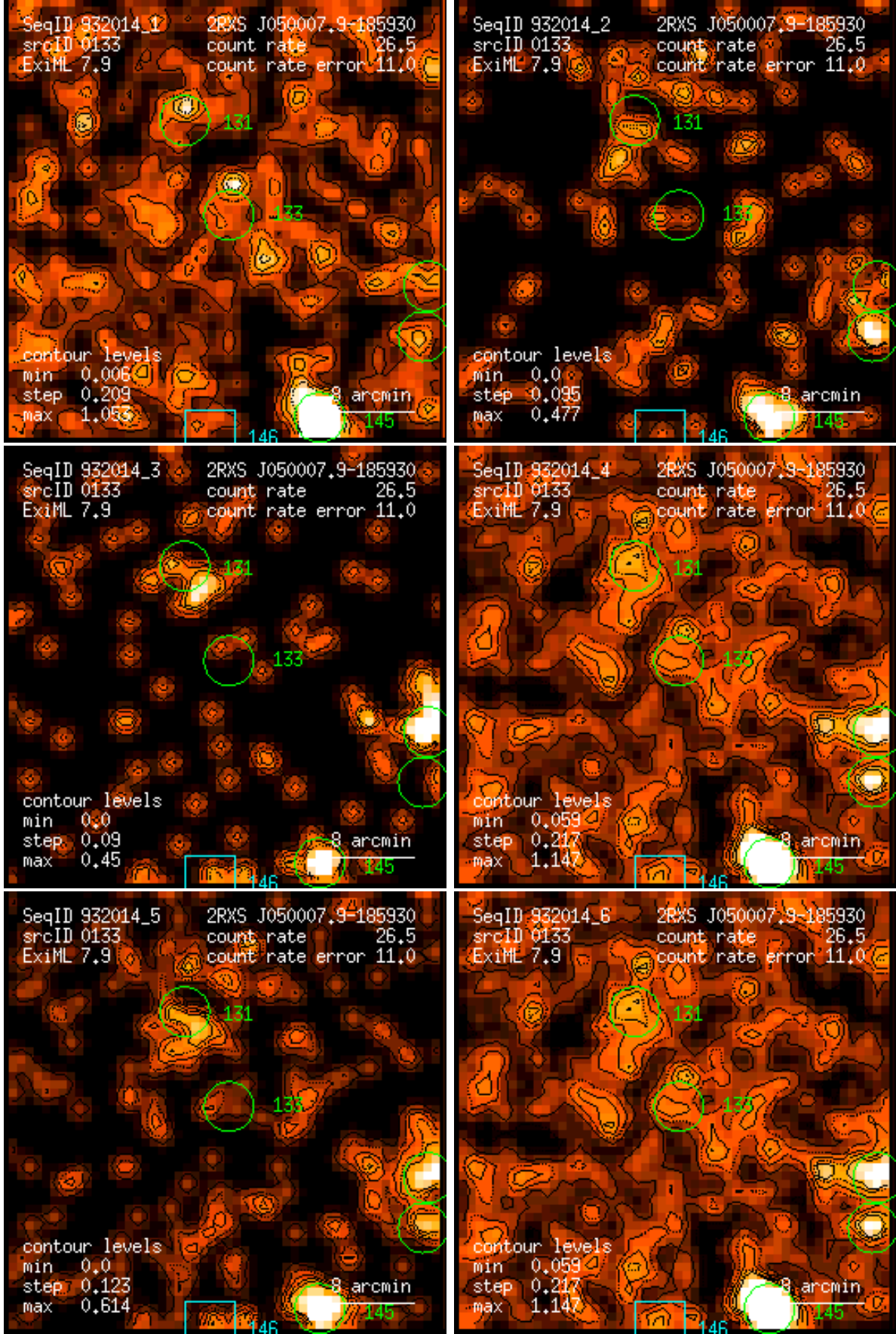
Figure 133: RASS 932014: detection 0133: band rate images, Gaussian filter: (1) PSPC channels 11 – 41, (2) 52 – 90, (3) 91 – 201, (4) 11 – 235, (5) 52 – 201, (6) 11 – 201. Broad band rates in counts/ks. Band rate contour levels in counts/ks/arcmin 2 .
