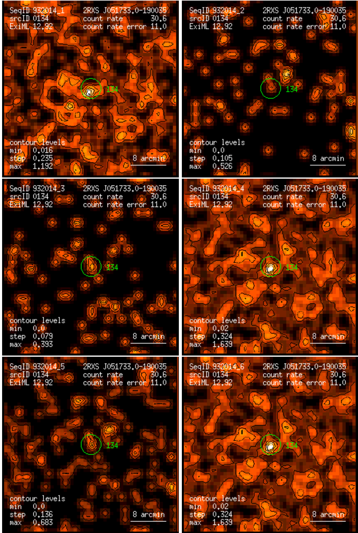
Figure 134: RASS 932014: detection 0134: band rate images, Gaussian filter: (1) PSPC channels 11 – 41, (2) 52 – 90, (3) 91 – 201, (4) 11 – 235, (5) 52 – 201, (6) 11 – 201. Broad band rates in counts/ks. Band rate contour levels in counts/ks/arcmin 2 .
