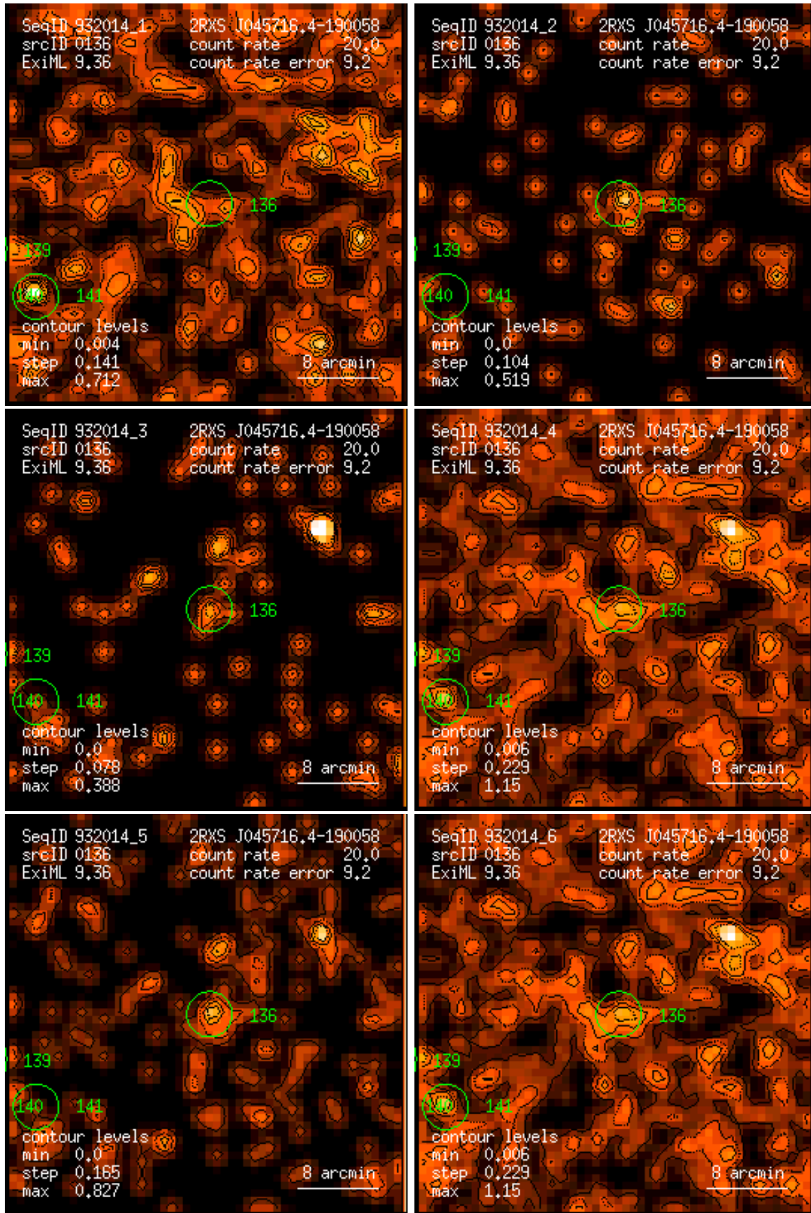
Figure 136: RASS 932014: detection 0136: band rate images, Gaussian filter: (1) PSPC channels 11 – 41, (2) 52 – 90, (3) 91 – 201, (4) 11 – 235, (5) 52 – 201, (6) 11 – 201. Broad band rates in counts/ks. Band rate contour levels in counts/ks/arcmin 2 .
