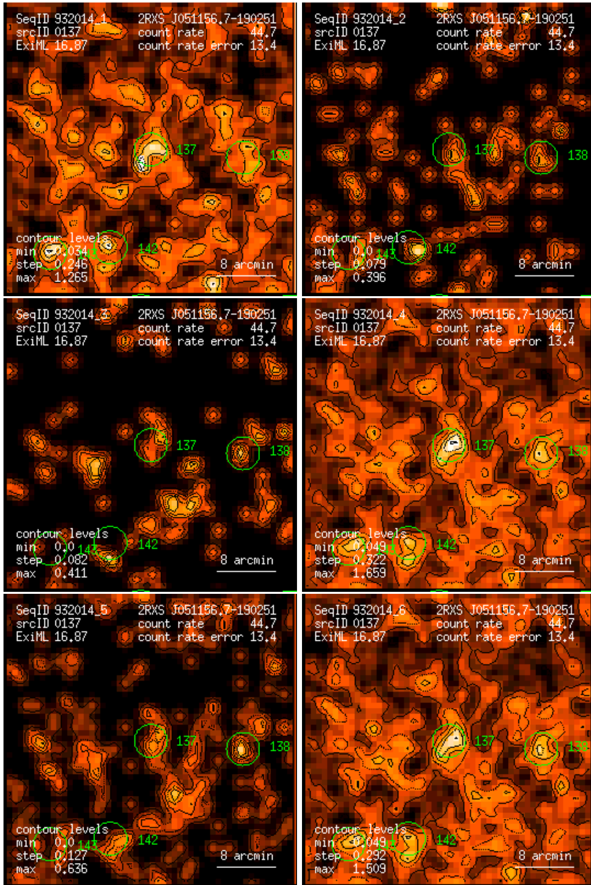
Figure 137: RASS 932014: detection 0137: band rate images, Gaussian filter: (1) PSPC channels 11 – 41, (2) 52 – 90, (3) 91 – 201, (4) 11 – 235, (5) 52 – 201, (6) 11 – 201. Broad band rates in counts/ks. Band rate contour levels in counts/ks/arcmin 2 .
