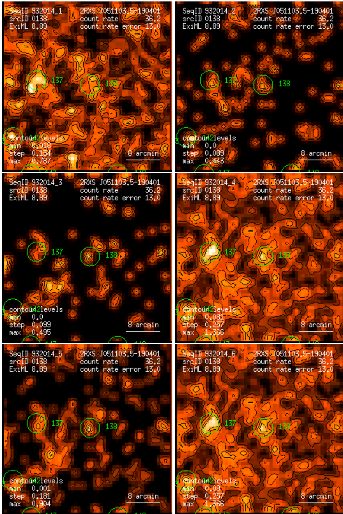
Figure 138: RASS 932014: detection 0138: band rate images, Gaussian filter: (1) PSPC channels 11 – 41, (2) 52 – 90, (3) 91 – 201, (4) 11 – 235, (5) 52 – 201, (6) 11 – 201. Broad band rates in counts/ks. Band rate contour levels in counts/ks/arcmin 2 .
