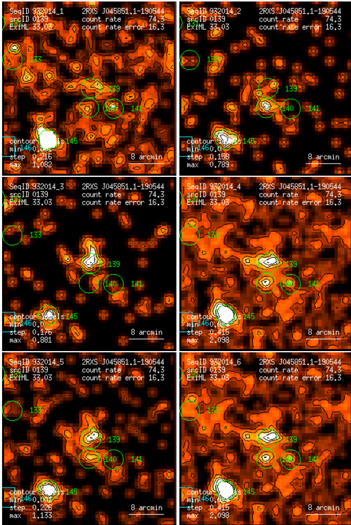
Figure 139: RASS 932014: detection 0139: band rate images, Gaussian filter: (1) PSPC channels 11 – 41, (2) 52 – 90, (3) 91 – 201, (4) 11 – 235, (5) 52 – 201, (6) 11 – 201. Broad band rates in counts/ks. Band rate contour levels in counts/ks/arcmin 2 .
