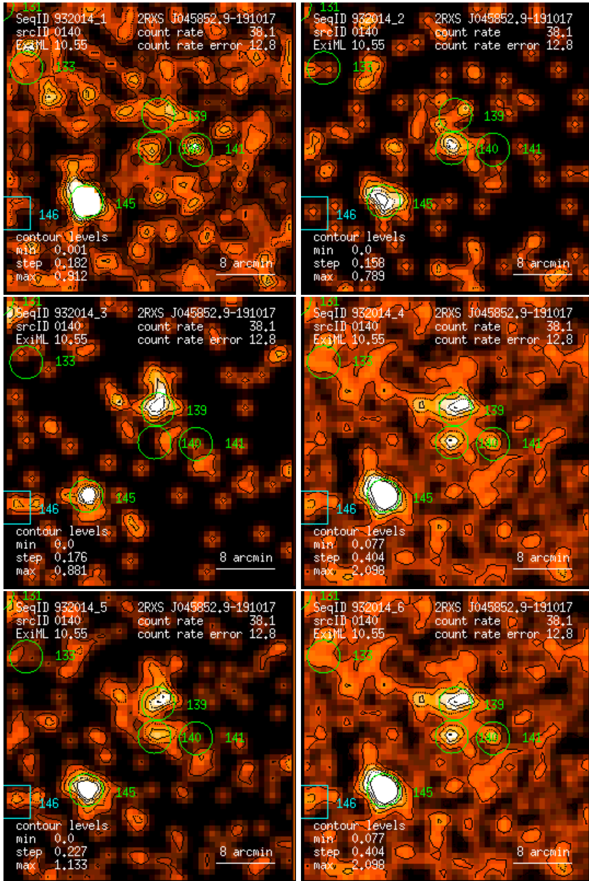
Figure 140: RASS 932014: detection 0140: band rate images, Gaussian filter: (1) PSPC channels 11 – 41, (2) 52 – 90, (3) 91 – 201, (4) 11 – 235, (5) 52 – 201, (6) 11 – 201. Broad band rates in counts/ks. Band rate contour levels in counts/ks/arcmin 2 .
