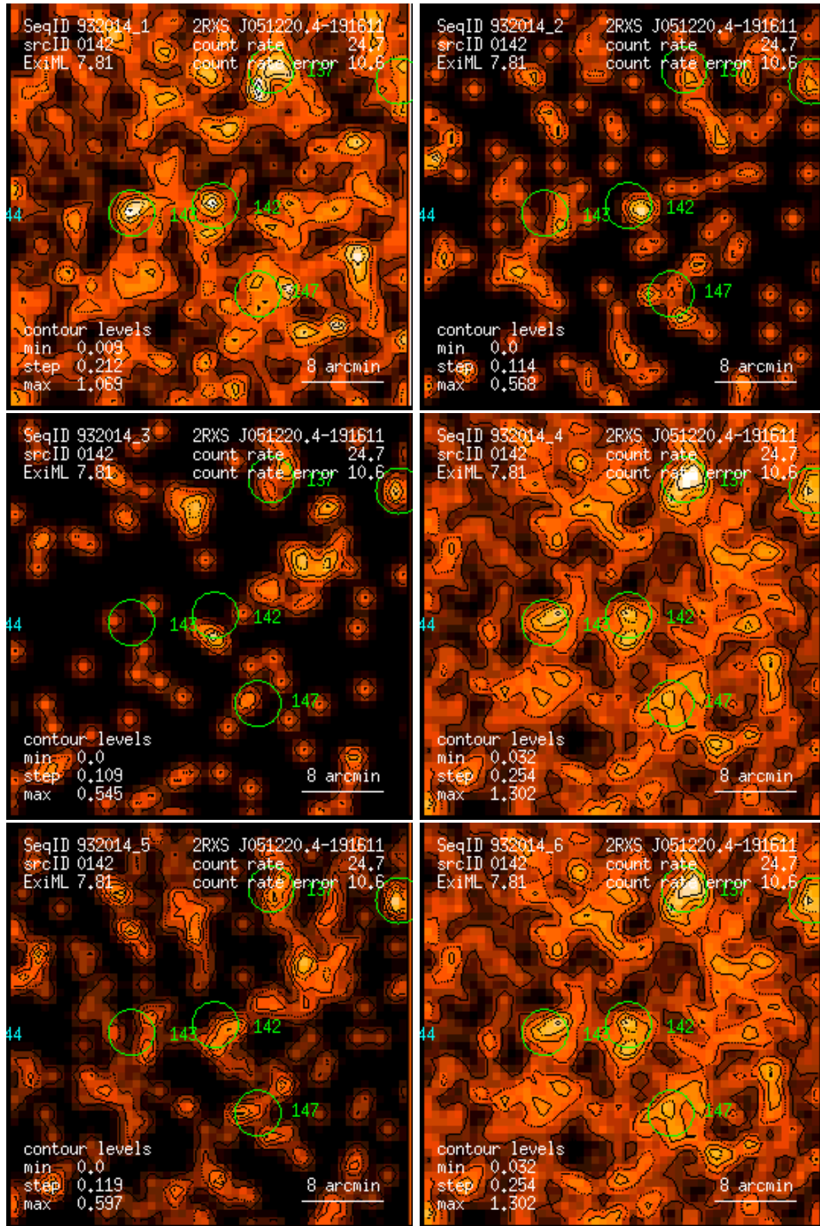
Figure 142: RASS 932014: detection 0142: band rate images, Gaussian filter: (1) PSPC channels 11 – 41, (2) 52 – 90, (3) 91 – 201, (4) 11 – 235, (5) 52 – 201, (6) 11 – 201. Broad band rates in counts/ks. Band rate contour levels in counts/ks/arcmin 2 .
