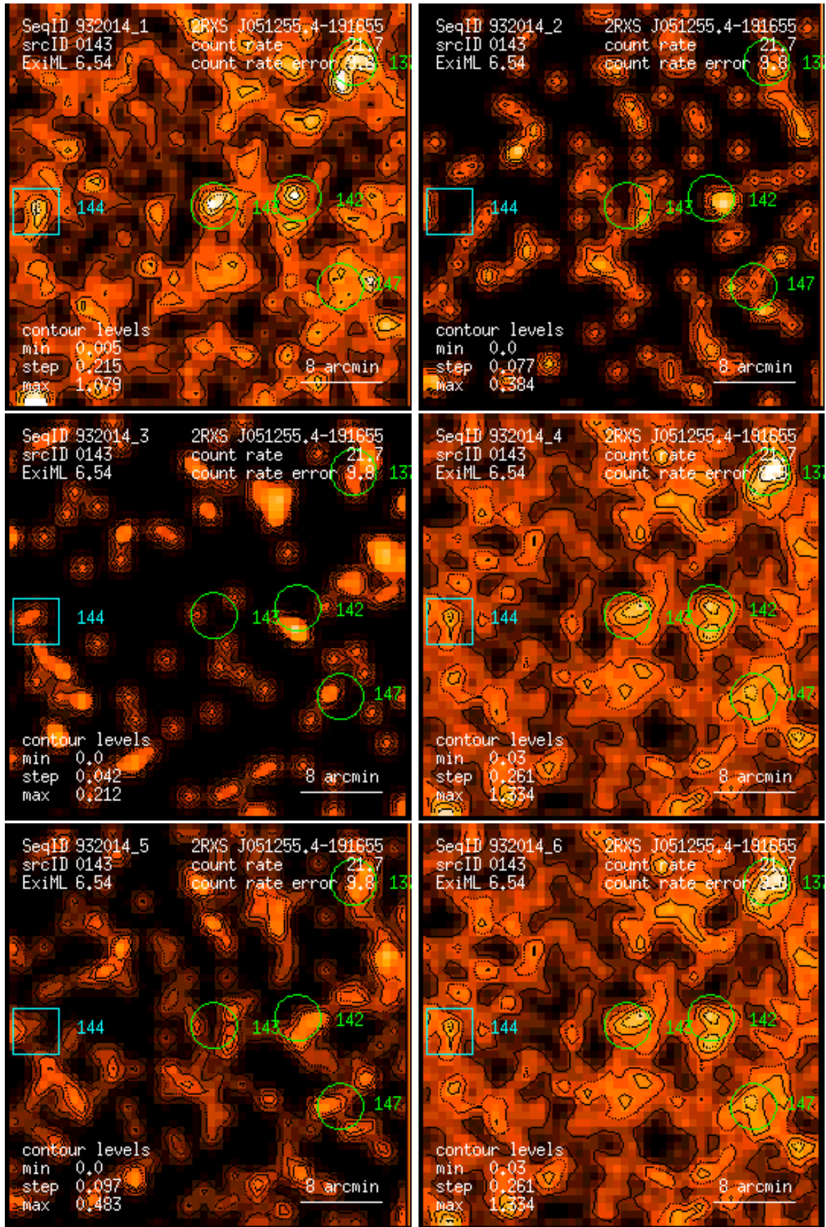
Figure 143: RASS 932014: detection 0143: band rate images, Gaussian filter: (1) PSPC channels 11 – 41, (2) 52 – 90, (3) 91 – 201, (4) 11 – 235, (5) 52 – 201, (6) 11 – 201. Broad band rates in counts/ks. Band rate contour levels in counts/ks/arcmin 2 .
