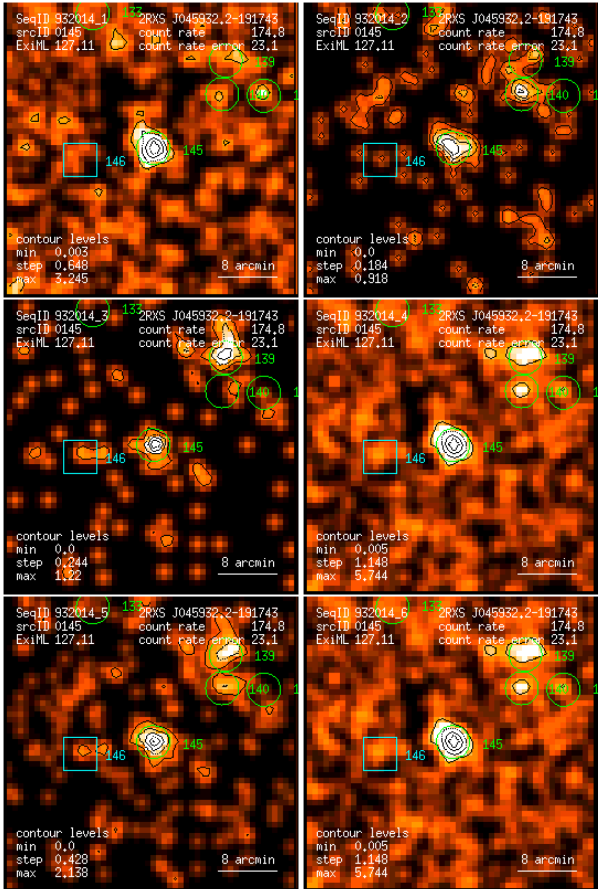
Figure 145: RASS 932014: detection 0145: band rate images, Gaussian filter: (1) PSPC channels 11 – 41, (2) 52 – 90, (3) 91 – 201, (4) 11 – 235, (5) 52 – 201, (6) 11 – 201. Broad band rates in counts/ks. Band rate contour levels in counts/ks/arcmin 2 .
