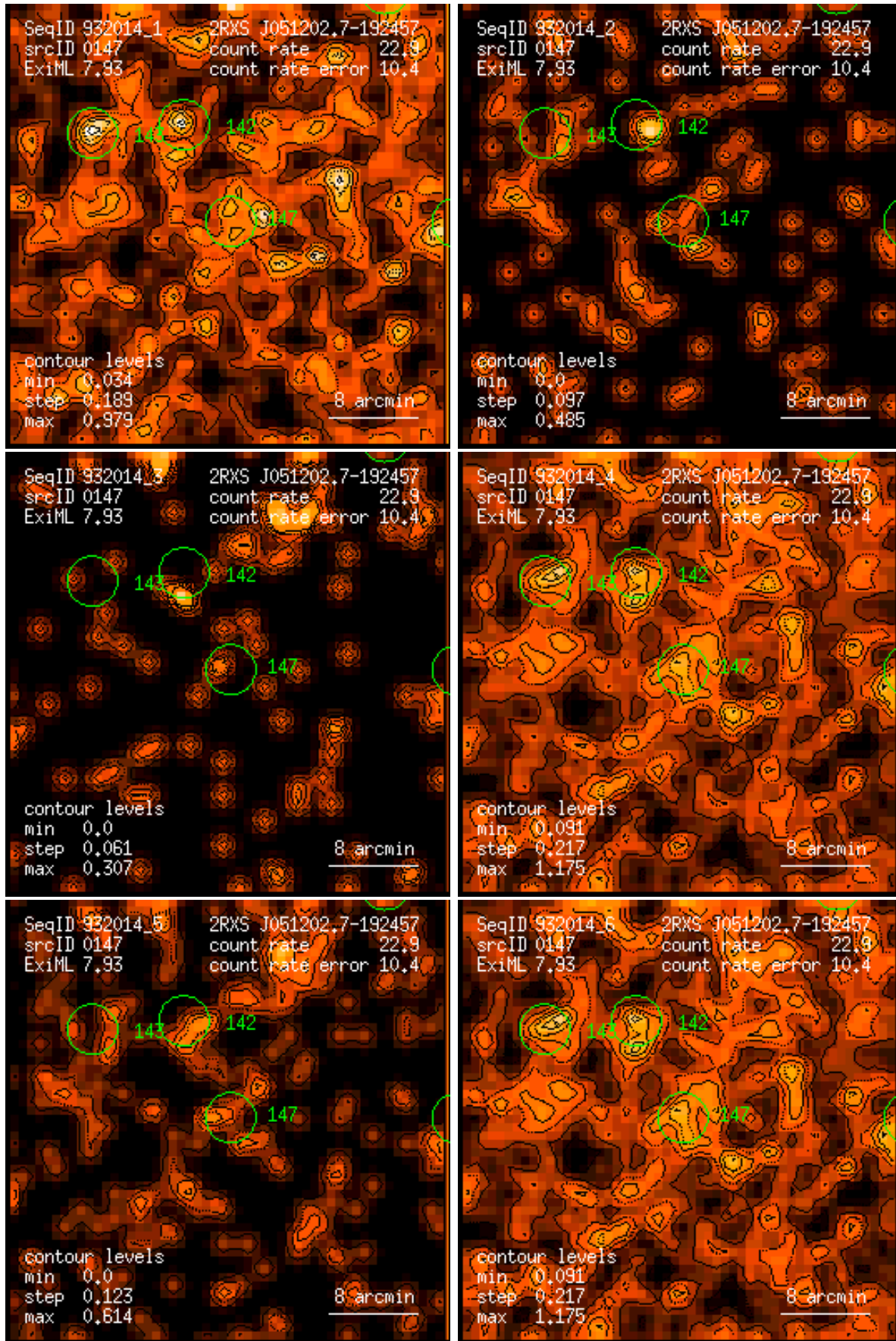
Figure 147: RASS 932014: detection 0147: band rate images, Gaussian filter: (1) PSPC channels 11 – 41, (2) 52 – 90, (3) 91 – 201, (4) 11 – 235, (5) 52 – 201, (6) 11 – 201. Broad band rates in counts/ks. Band rate contour levels in counts/ks/arcmin 2 .
