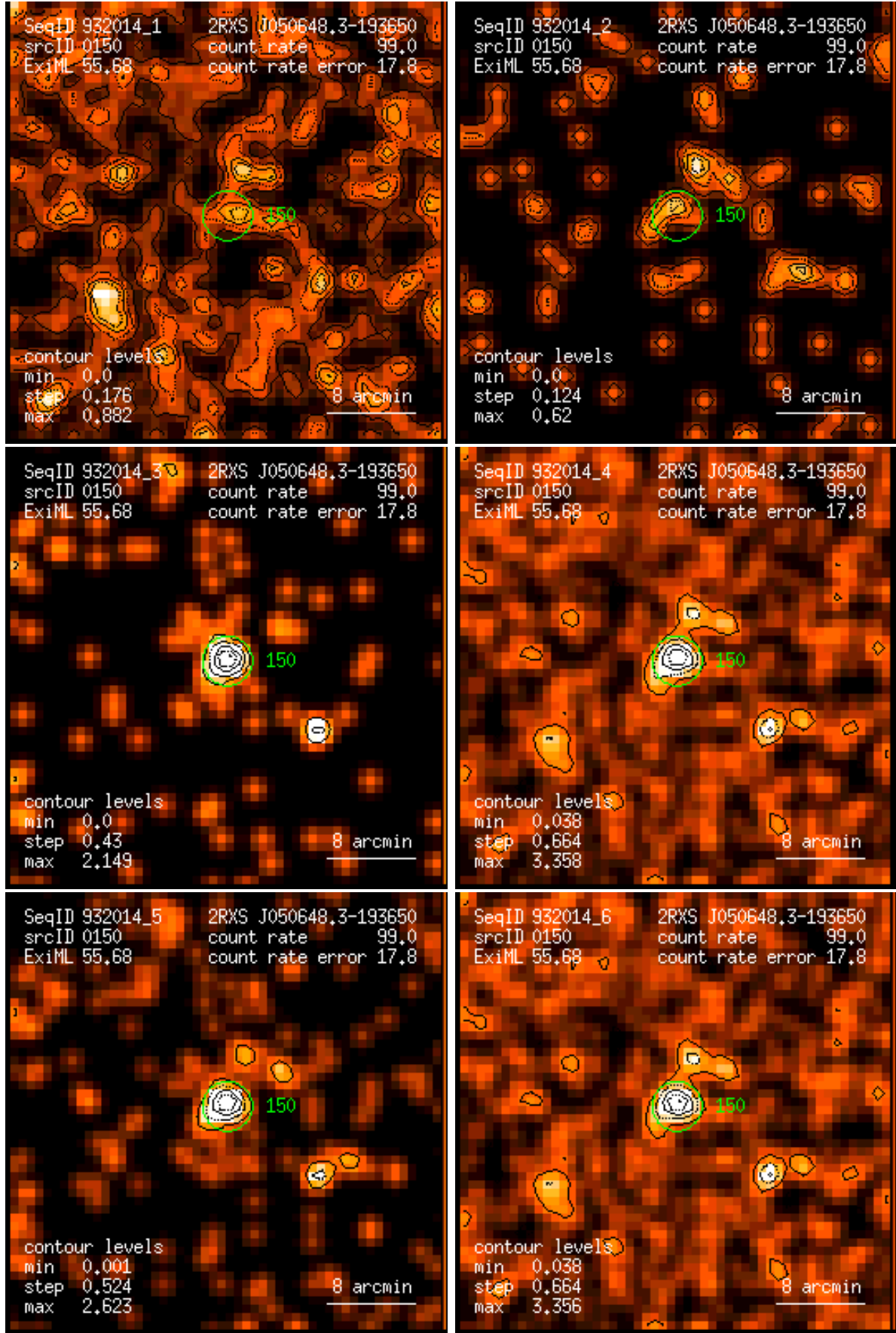
Figure 150: RASS 932014: detection 0150: band rate images, Gaussian filter: (1) PSPC channels 11 – 41, (2) 52 – 90, (3) 91 – 201, (4) 11 – 235, (5) 52 – 201, (6) 11 – 201. Broad band rates in counts/ks. Band rate contour levels in counts/ks/arcmin 2 .
