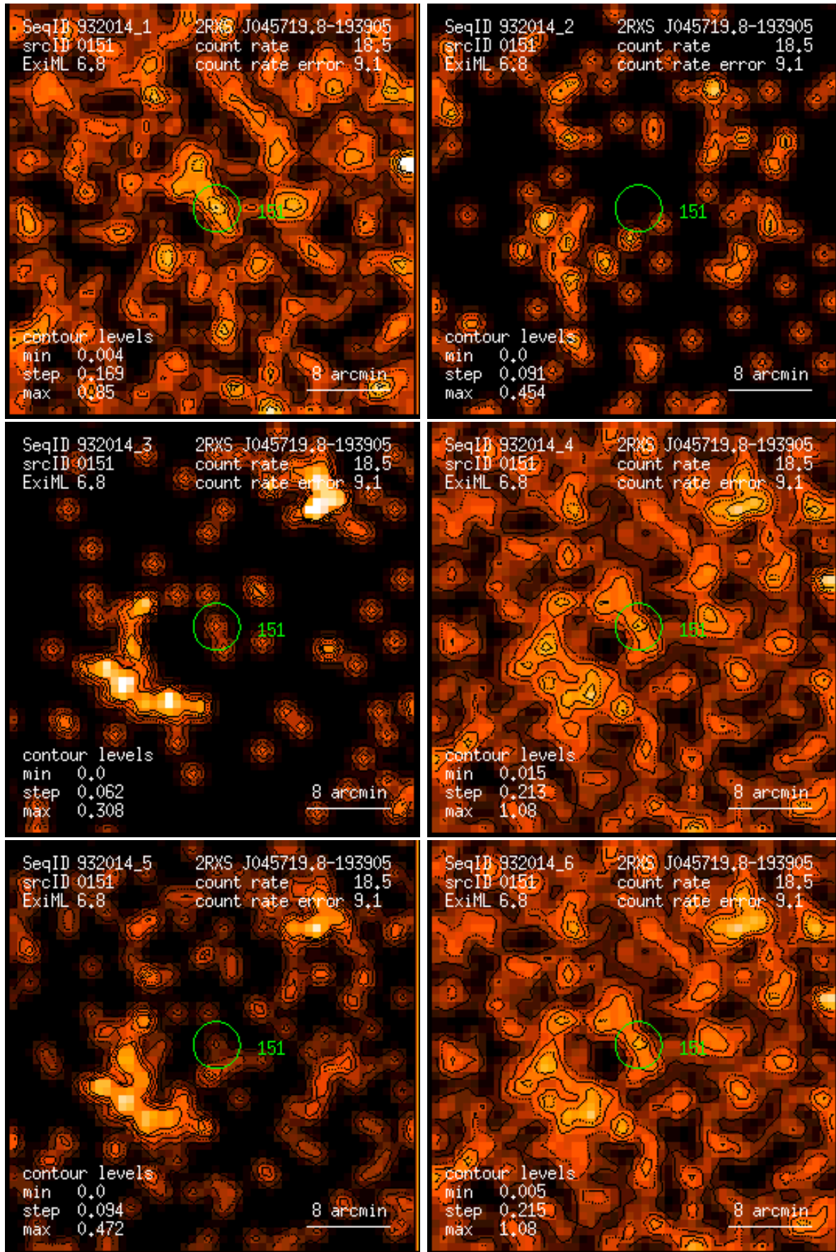
Figure 151: RASS 932014: detection 0151: band rate images, Gaussian filter: (1) PSPC channels 11 – 41, (2) 52 – 90, (3) 91 – 201, (4) 11 – 235, (5) 52 – 201, (6) 11 – 201. Broad band rates in counts/ks. Band rate contour levels in counts/ks/arcmin 2 .
