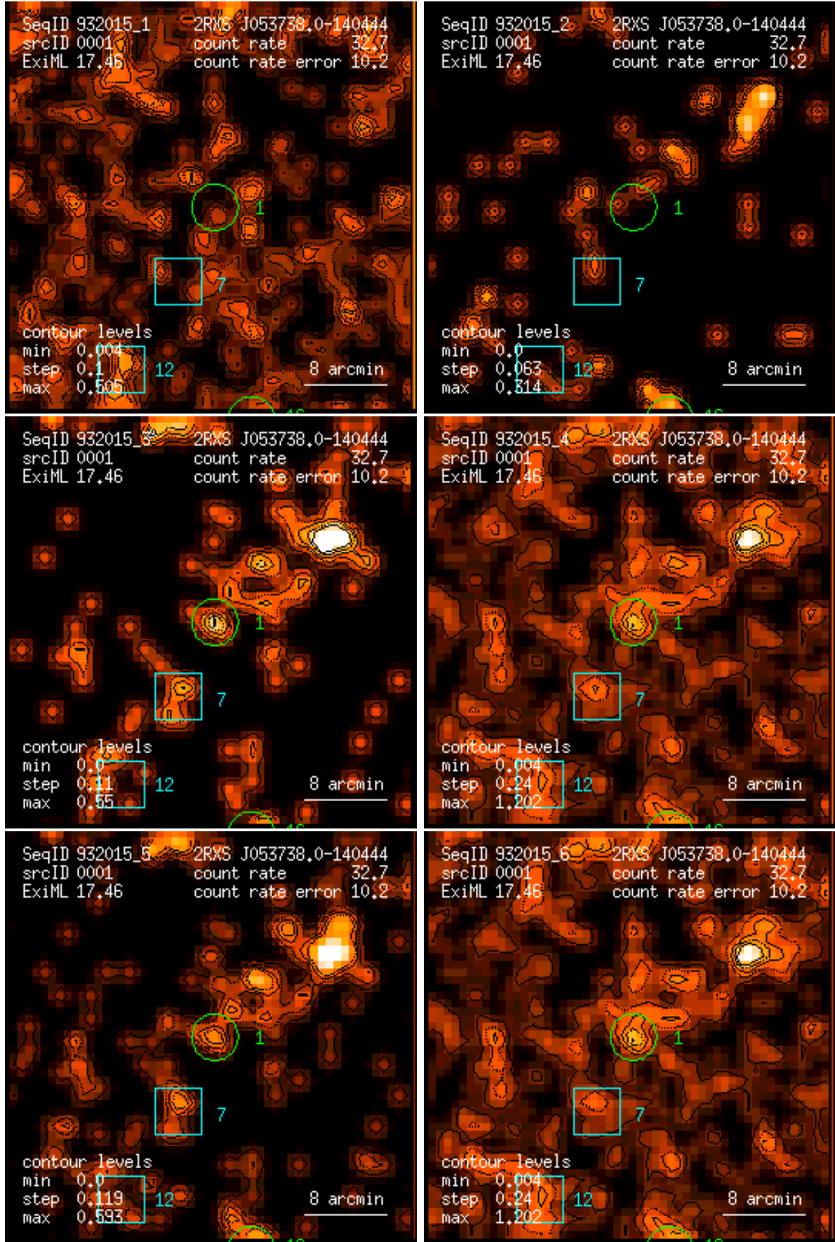
Figure 1: RASS 932015: detection 0001: band rate images, Gaussian filter: (1) PSPC channels 11 – 41, (2) 52 – 90, (3) 91 – 201, (4) 11 – 235, (5) 52 – 201, (6) 11 – 201. Broad band rates in counts/ks. Band rate contour levels in counts/ks/arcmin 2 .
