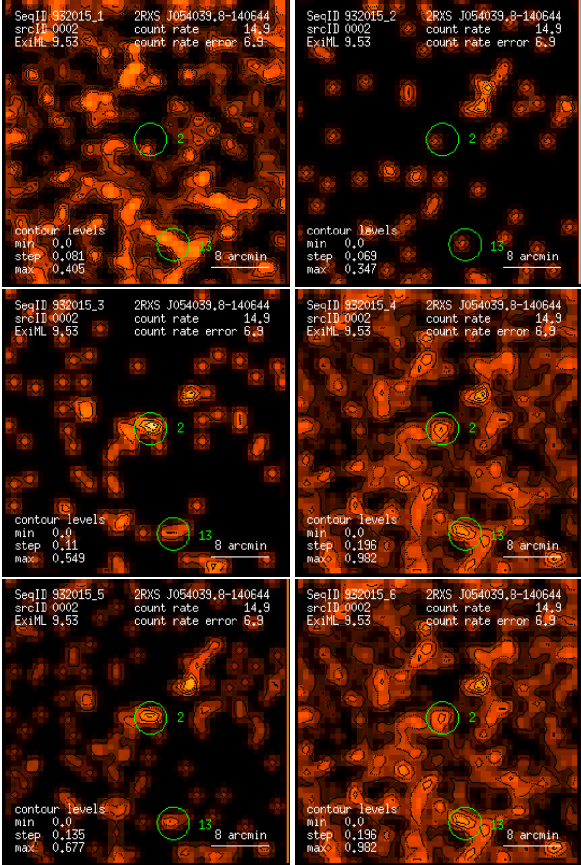
Figure 2: RASS 932015: detection 0002: band rate images, Gaussian filter: (1) PSPC channels 11 – 41, (2) 52 – 90, (3) 91 – 201, (4) 11 – 235, (5) 52 – 201, (6) 11 – 201. Broad band rates in counts/ks. Band rate contour levels in counts/ks/arcmin 2 .
