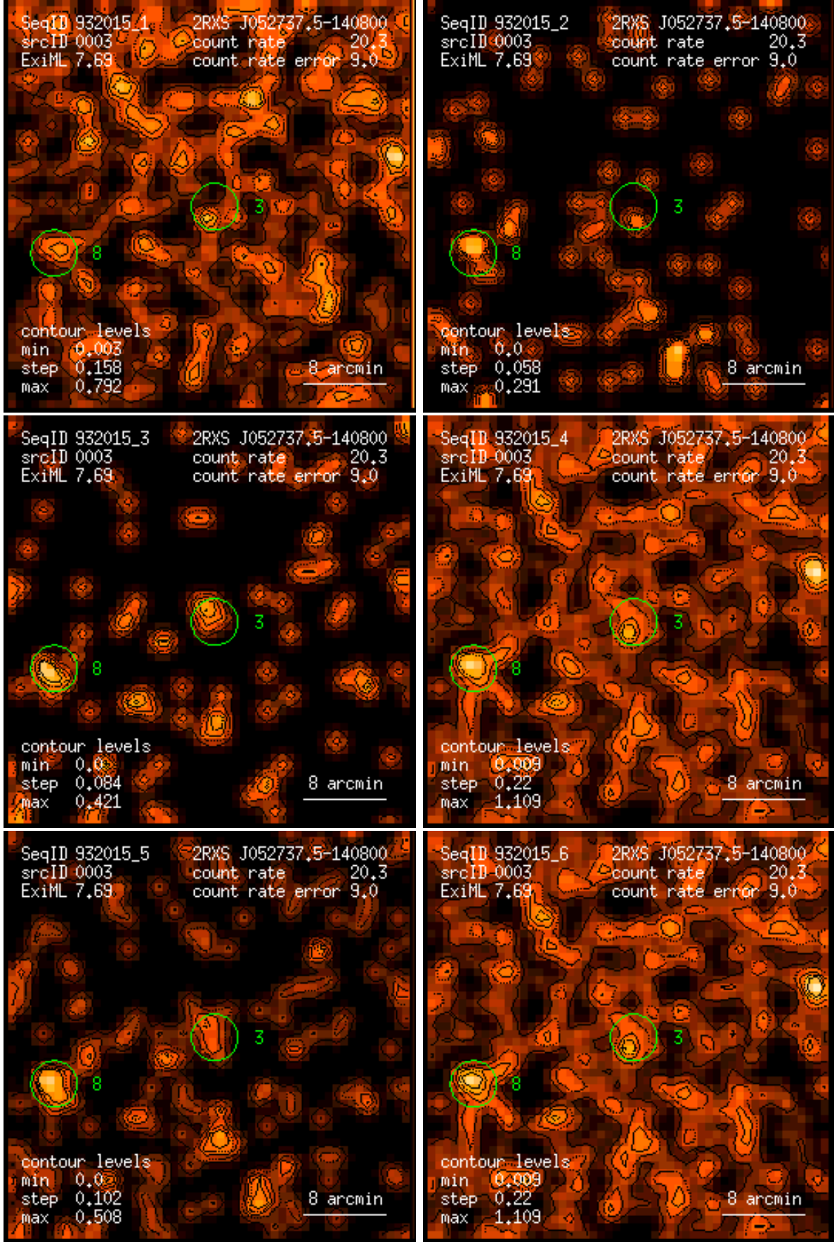
Figure 3: RASS 932015: detection 0003: band rate images, Gaussian filter: (1) PSPC channels 11 – 41, (2) 52 – 90, (3) 91 – 201, (4) 11 – 235, (5) 52 – 201, (6) 11 – 201. Broad band rates in counts/ks. Band rate contour levels in counts/ks/arcmin 2 .
