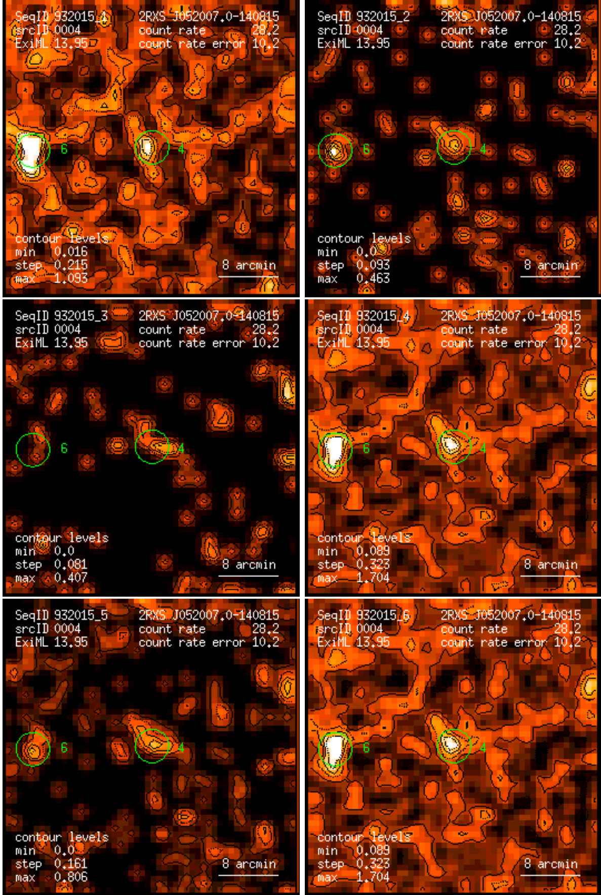
Figure 4: RASS 932015: detection 0004: band rate images, Gaussian filter: (1) PSPC channels 11 – 41, (2) 52 – 90, (3) 91 – 201, (4) 11 – 235, (5) 52 – 201, (6) 11 – 201. Broad band rates in counts/ks. Band rate contour levels in counts/ks/arcmin 2 .
