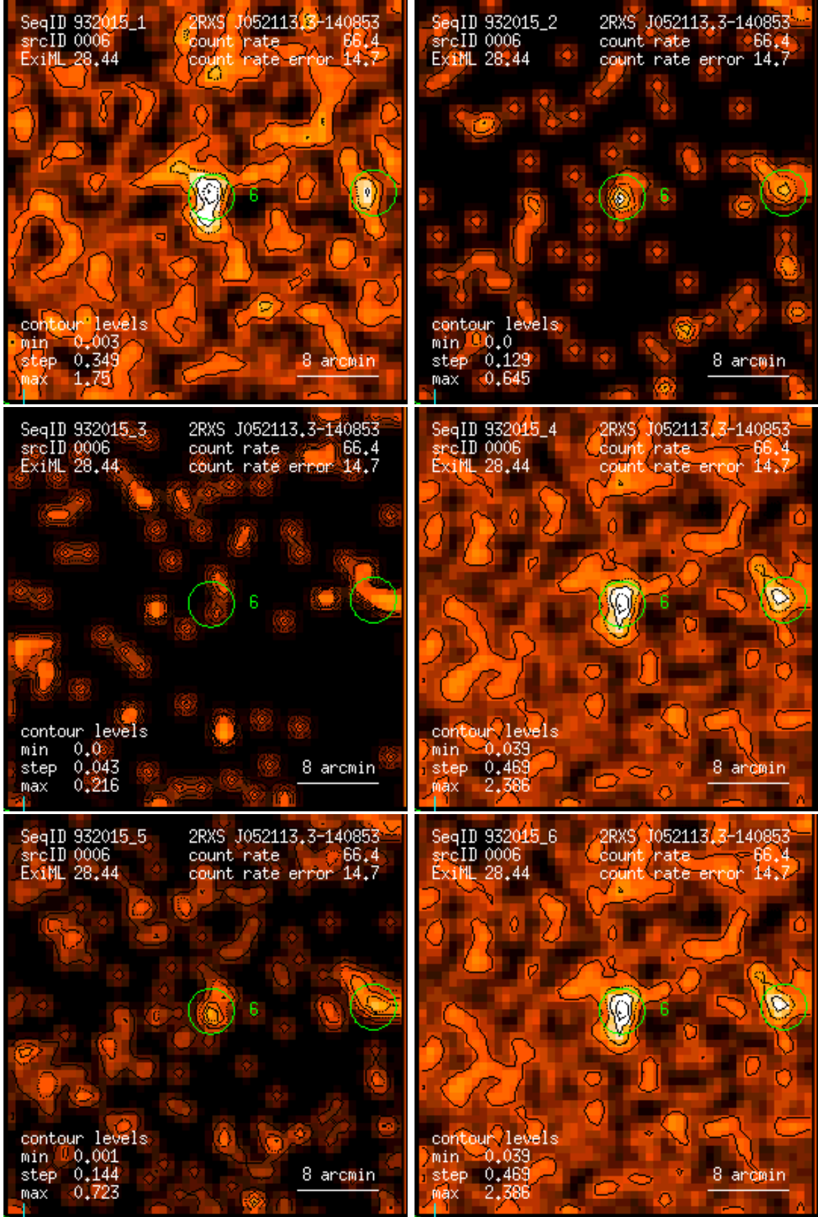
Figure 6: RASS 932015: detection 0006: band rate images, Gaussian filter: (1) PSPC channels 11 – 41, (2) 52 – 90, (3) 91 – 201, (4) 11 – 235, (5) 52 – 201, (6) 11 – 201. Broad band rates in counts/ks. Band rate contour levels in counts/ks/arcmin 2 .
