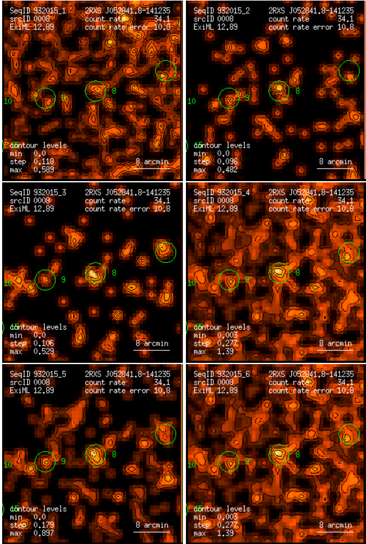
Figure 8: RASS 932015: detection 0008: band rate images, Gaussian filter: (1) PSPC channels 11 – 41, (2) 52 – 90, (3) 91 – 201, (4) 11 – 235, (5) 52 – 201, (6) 11 – 201. Broad band rates in counts/ks. Band rate contour levels in counts/ks/arcmin 2 .
