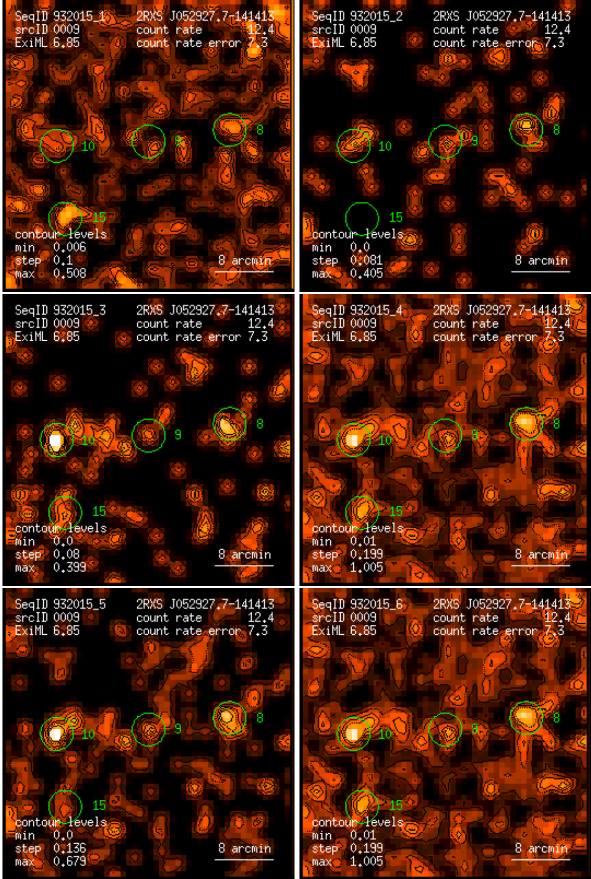
Figure 9: RASS 932015: detection 0009: band rate images, Gaussian filter: (1) PSPC channels 11 – 41, (2) 52 – 90, (3) 91 – 201, (4) 11 – 235, (5) 52 – 201, (6) 11 – 201. Broad band rates in counts/ks. Band rate contour levels in counts/ks/arcmin 2 .
