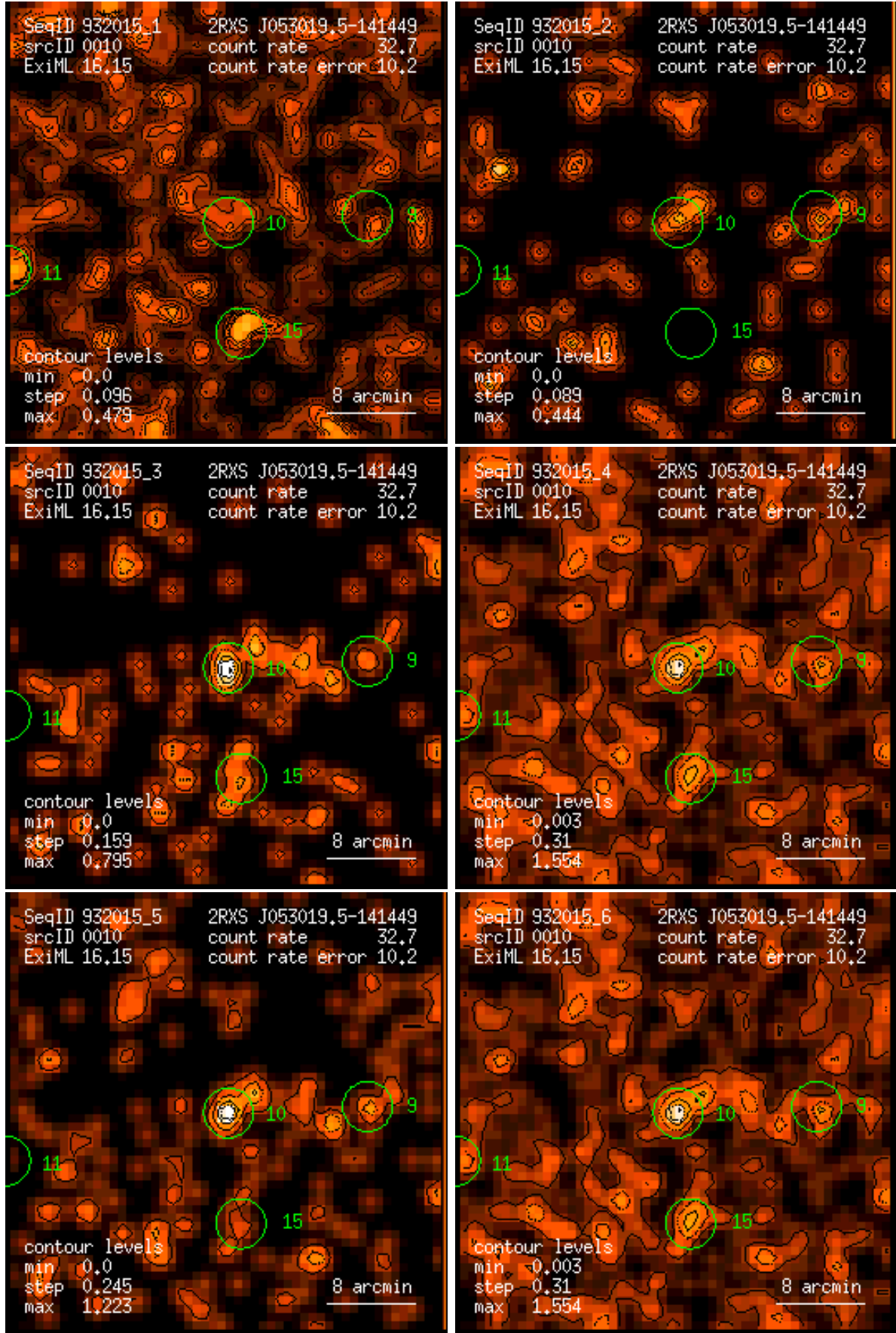
Figure 10: RASS 932015: detection 0010: band rate images, Gaussian filter: (1) PSPC channels 11 – 41, (2) 52 – 90, (3) 91 – 201, (4) 11 – 235, (5) 52 – 201, (6) 11 – 201. Broad band rates in counts/ks. Band rate contour levels in counts/ks/arcmin 2 .
