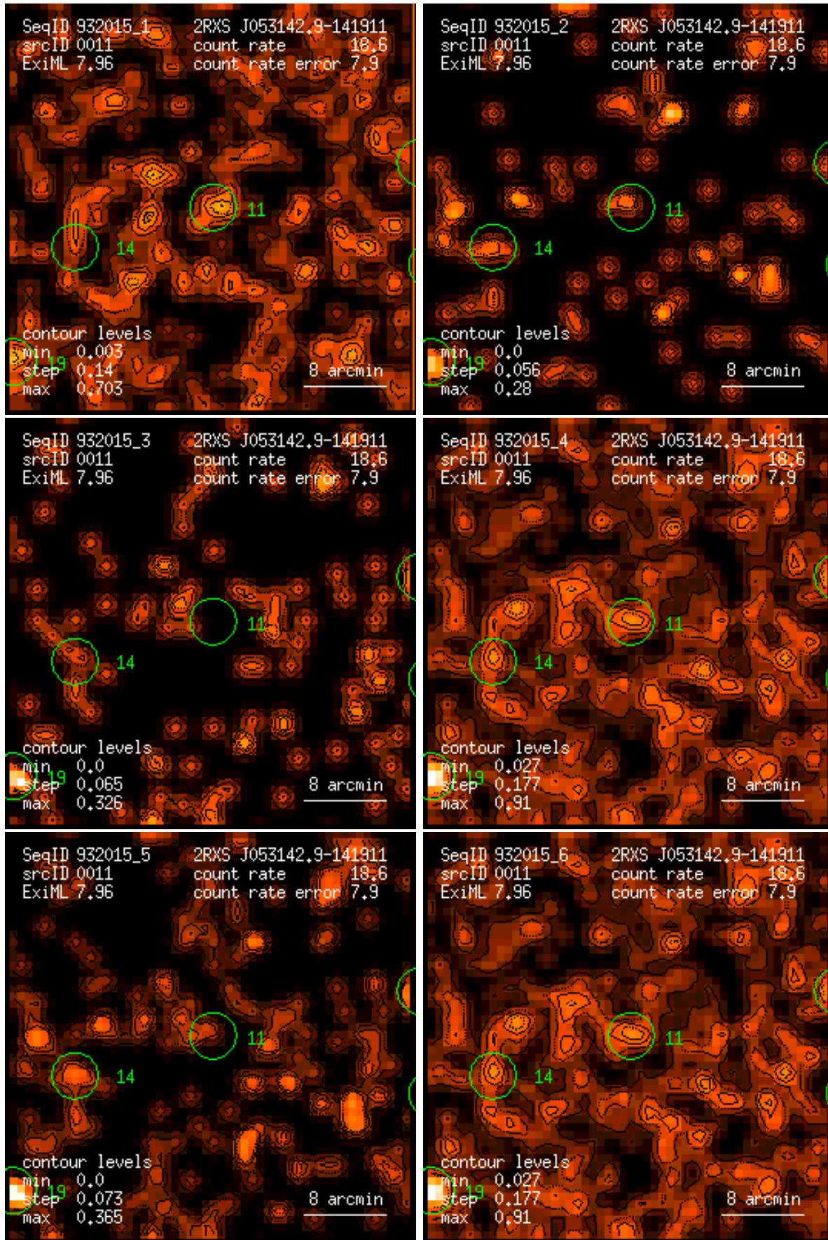
Figure 11: RASS 932015: detection 0011: band rate images, Gaussian filter: (1) PSPC channels 11 – 41, (2) 52 – 90, (3) 91 – 201, (4) 11 – 235, (5) 52 – 201, (6) 11 – 201. Broad band rates in counts/ks. Band rate contour levels in counts/ks/arcmin 2 .
