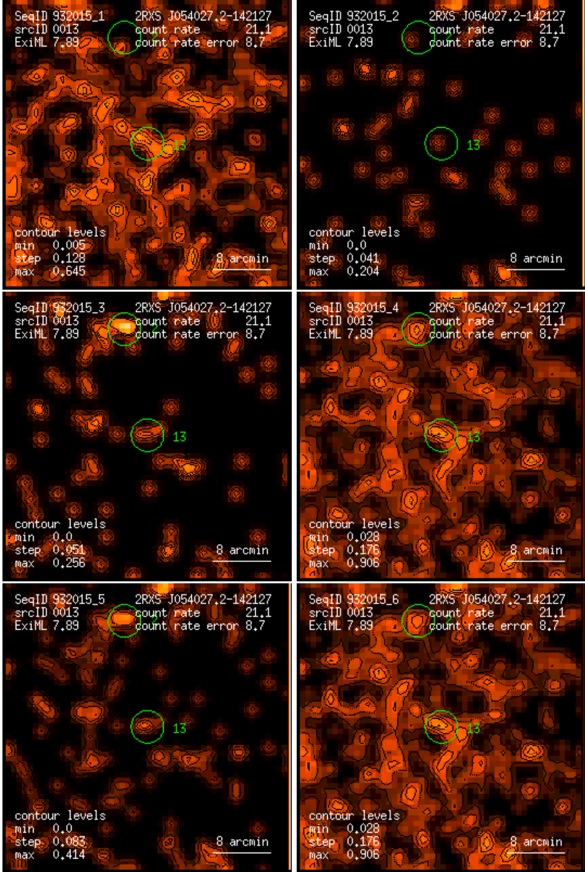
Figure 13: RASS 932015: detection 0013: band rate images, Gaussian filter: (1) PSPC channels 11 – 41, (2) 52 – 90, (3) 91 – 201, (4) 11 – 235, (5) 52 – 201, (6) 11 – 201. Broad band rates in counts/ks. Band rate contour levels in counts/ks/arcmin 2 .
