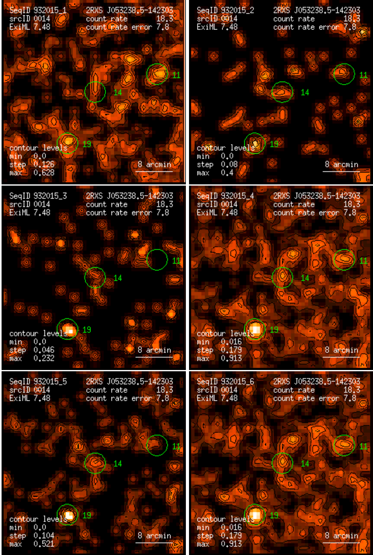
Figure 14: RASS 932015: detection 0014: band rate images, Gaussian filter: (1) PSPC channels 11 – 41, (2) 52 – 90, (3) 91 – 201, (4) 11 – 235, (5) 52 – 201, (6) 11 – 201. Broad band rates in counts/ks. Band rate contour levels in counts/ks/arcmin 2 .
