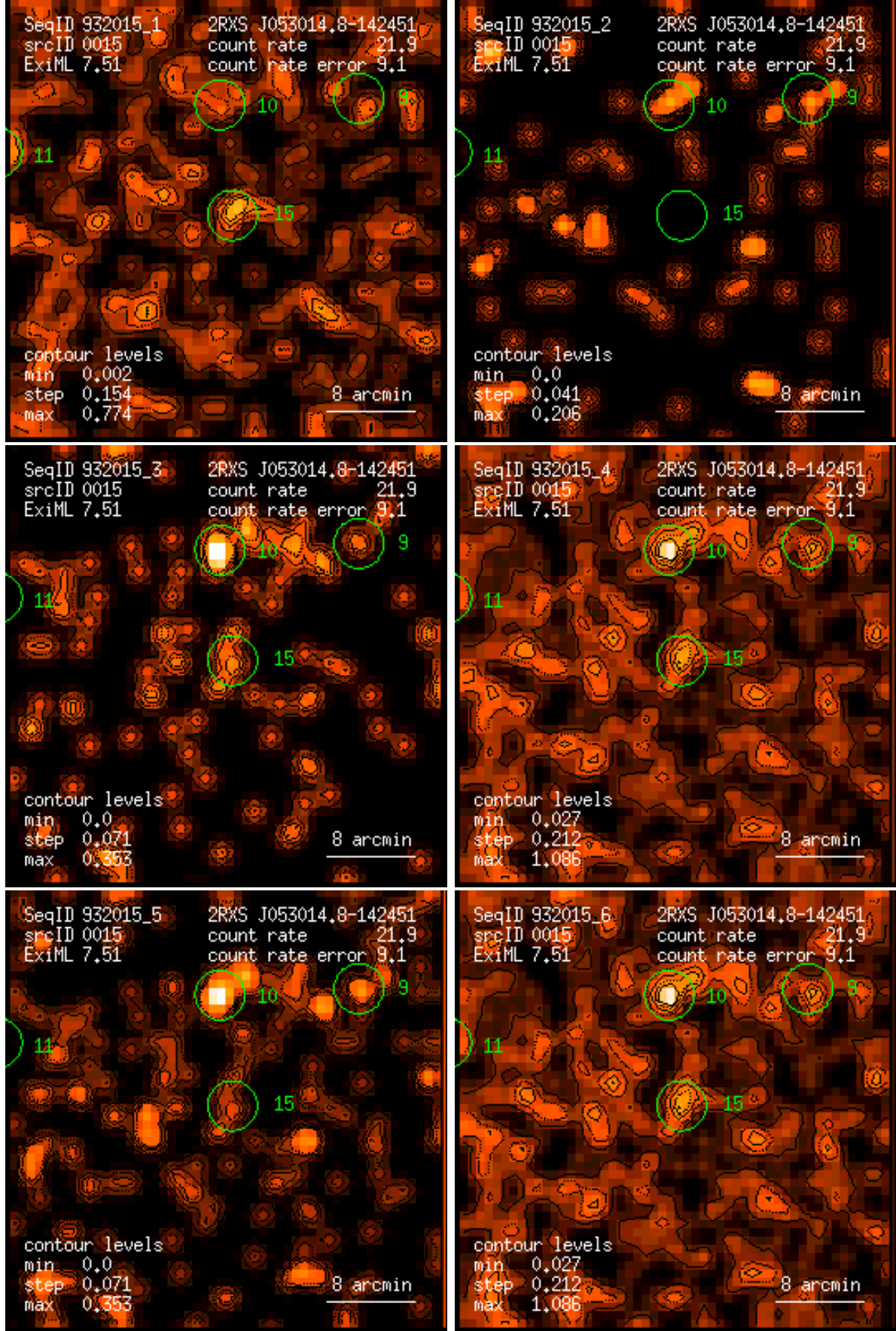
Figure 15: RASS 932015: detection 0015: band rate images, Gaussian filter: (1) PSPC channels 11 – 41, (2) 52 – 90, (3) 91 – 201, (4) 11 – 235, (5) 52 – 201, (6) 11 – 201. Broad band rates in counts/ks. Band rate contour levels in counts/ks/arcmin 2 .
