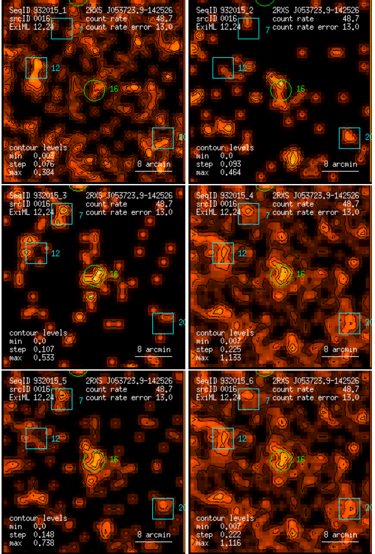
Figure 16: RASS 932015: detection 0016: band rate images, Gaussian filter: (1) PSPC channels 11 – 41, (2) 52 – 90, (3) 91 – 201, (4) 11 – 235, (5) 52 – 201, (6) 11 – 201. Broad band rates in counts/ks. Band rate contour levels in counts/ks/arcmin 2 .
