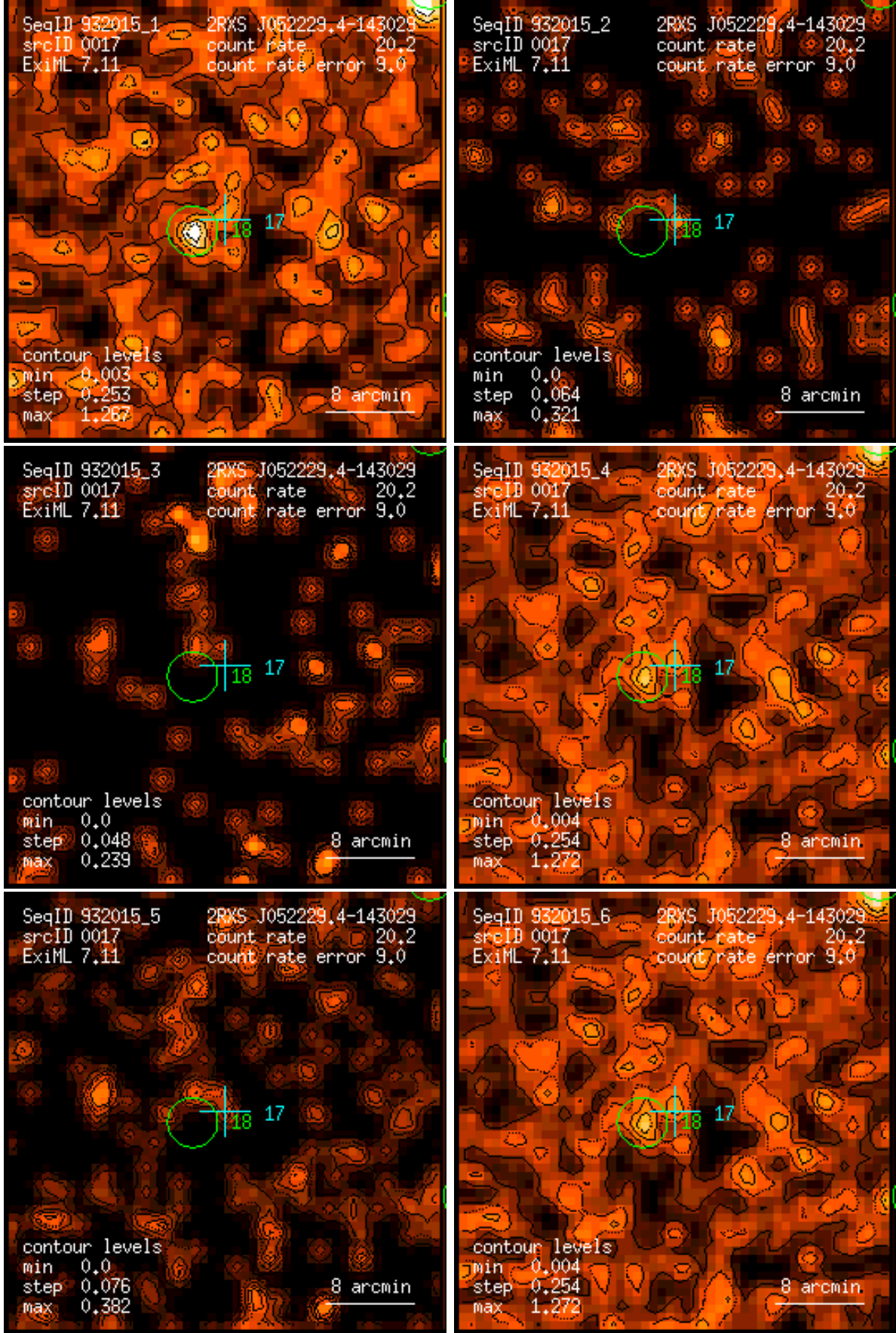
Figure 17: RASS 932015: detection 0017: band rate images, Gaussian filter: (1) PSPC channels 11 – 41, (2) 52 – 90, (3) 91 – 201, (4) 11 – 235, (5) 52 – 201, (6) 11 – 201. Broad band rates in counts/ks. Band rate contour levels in counts/ks/arcmin 2 .
