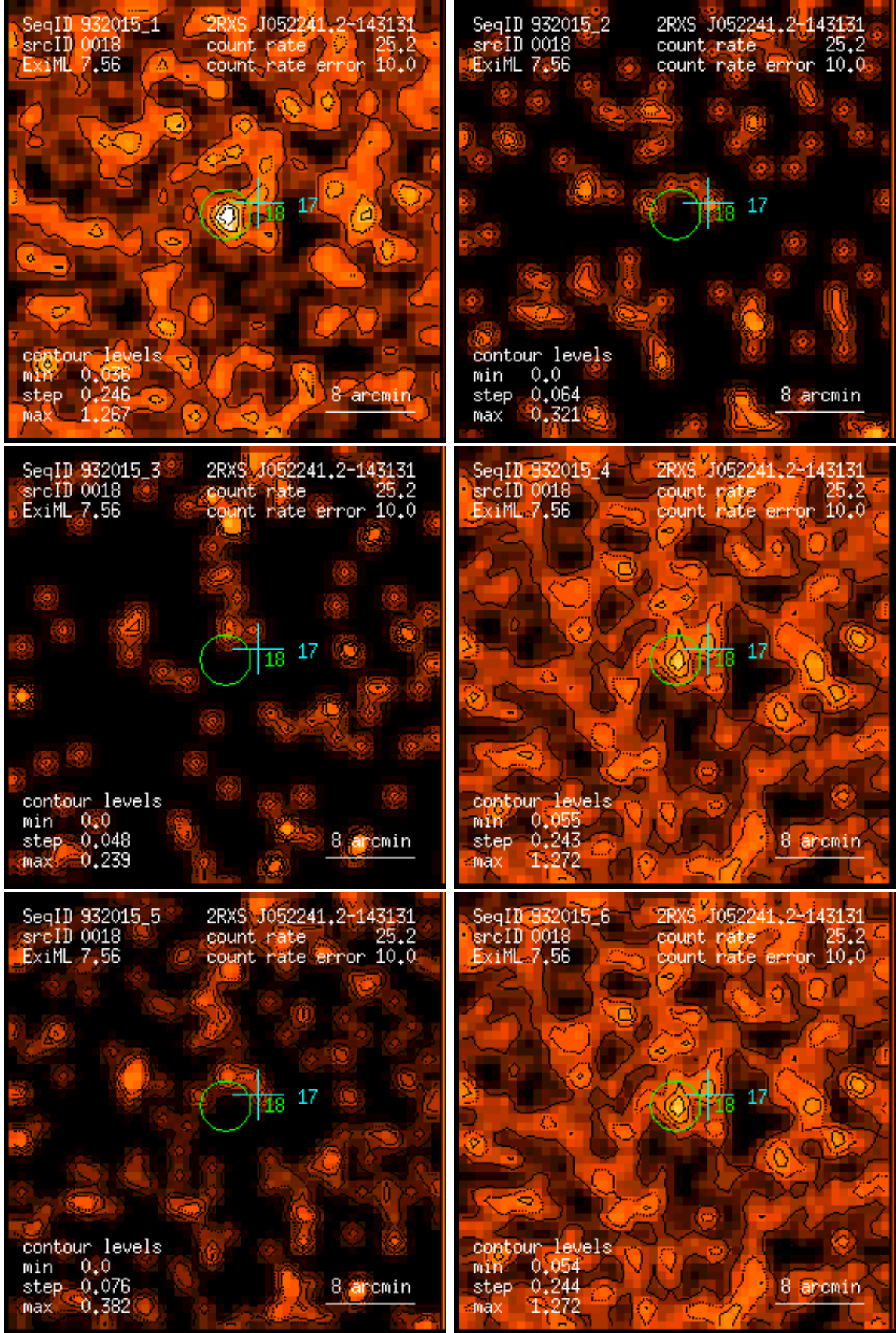
Figure 18: RASS 932015: detection 0018: band rate images, Gaussian filter: (1) PSPC channels 11 – 41, (2) 52 – 90, (3) 91 – 201, (4) 11 – 235, (5) 52 – 201, (6) 11 – 201. Broad band rates in counts/ks. Band rate contour levels in counts/ks/arcmin 2 .
