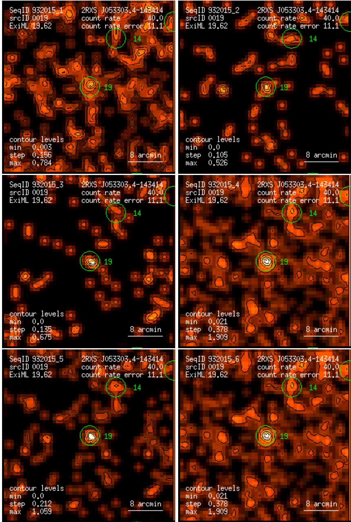
Figure 19: RASS 932015: detection 0019: band rate images, Gaussian filter: (1) PSPC channels 11 – 41, (2) 52 – 90, (3) 91 – 201, (4) 11 – 235, (5) 52 – 201, (6) 11 – 201. Broad band rates in counts/ks. Band rate contour levels in counts/ks/arcmin 2 .
