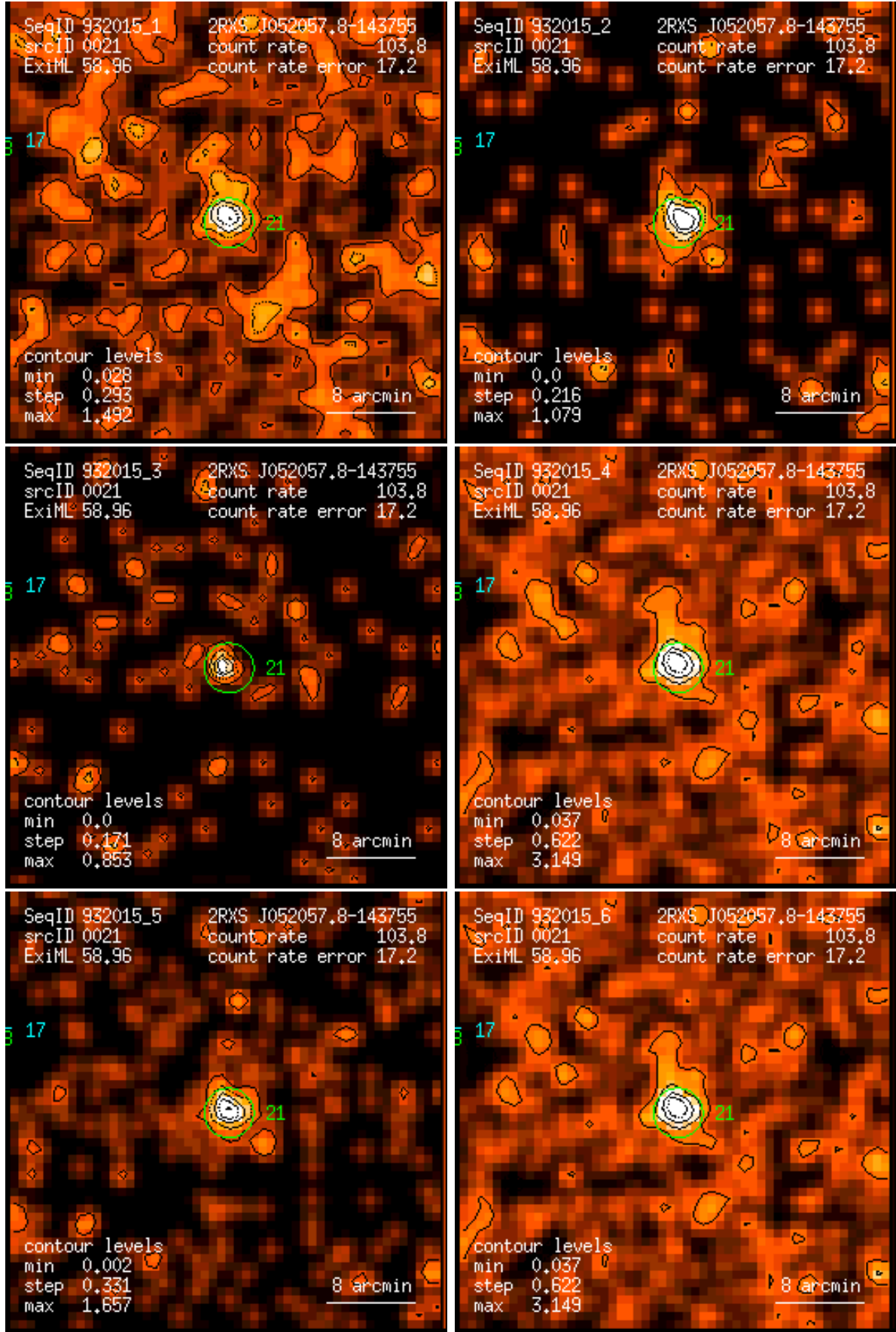
Figure 21: RASS 932015: detection 0021: band rate images, Gaussian filter: (1) PSPC channels 11 – 41, (2) 52 – 90, (3) 91 – 201, (4) 11 – 235, (5) 52 – 201, (6) 11 – 201. Broad band rates in counts/ks. Band rate contour levels in counts/ks/arcmin 2 .
