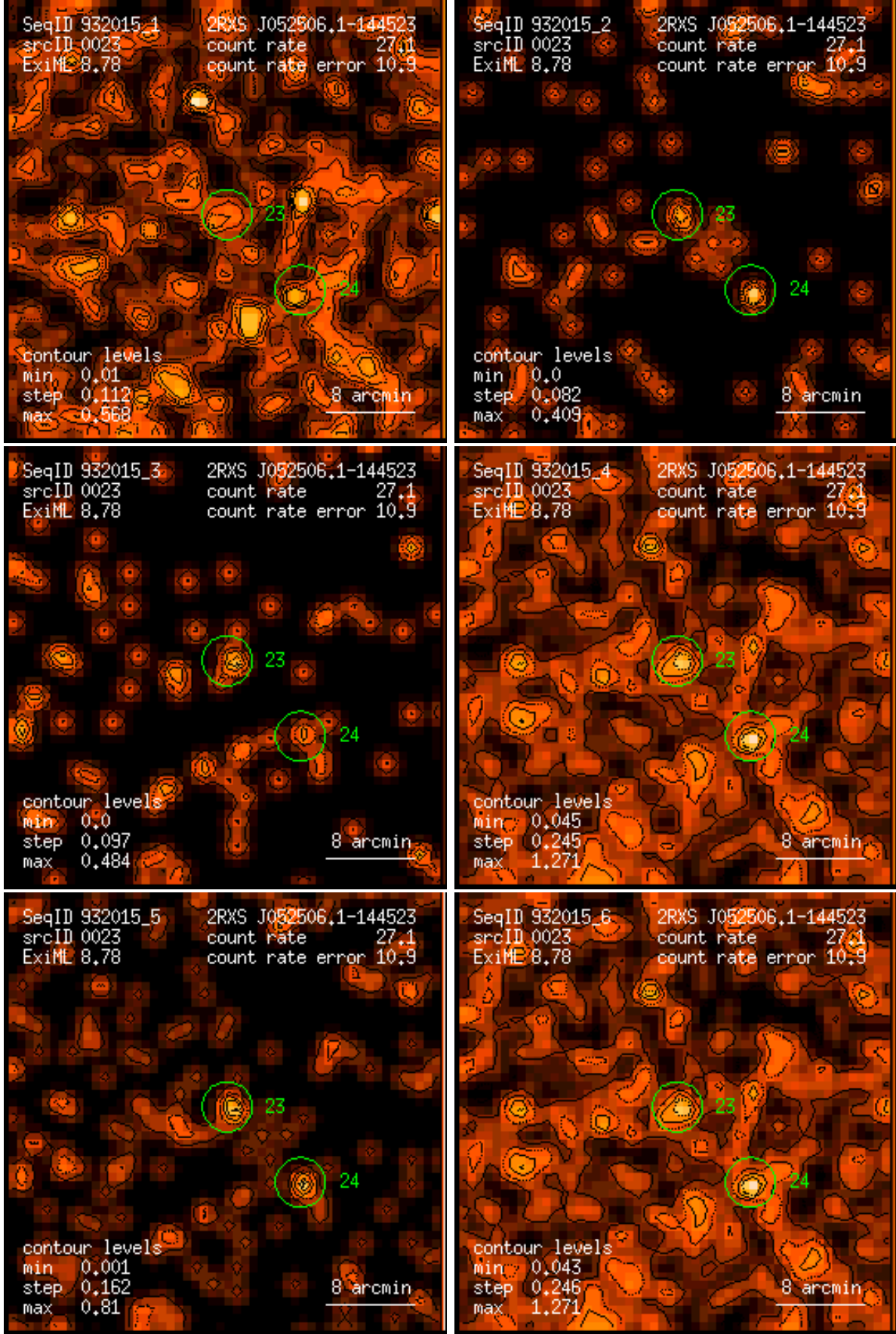
Figure 23: RASS 932015: detection 0023: band rate images, Gaussian filter: (1) PSPC channels 11 – 41, (2) 52 – 90, (3) 91 – 201, (4) 11 – 235, (5) 52 – 201, (6) 11 – 201. Broad band rates in counts/ks. Band rate contour levels in counts/ks/arcmin 2 .
