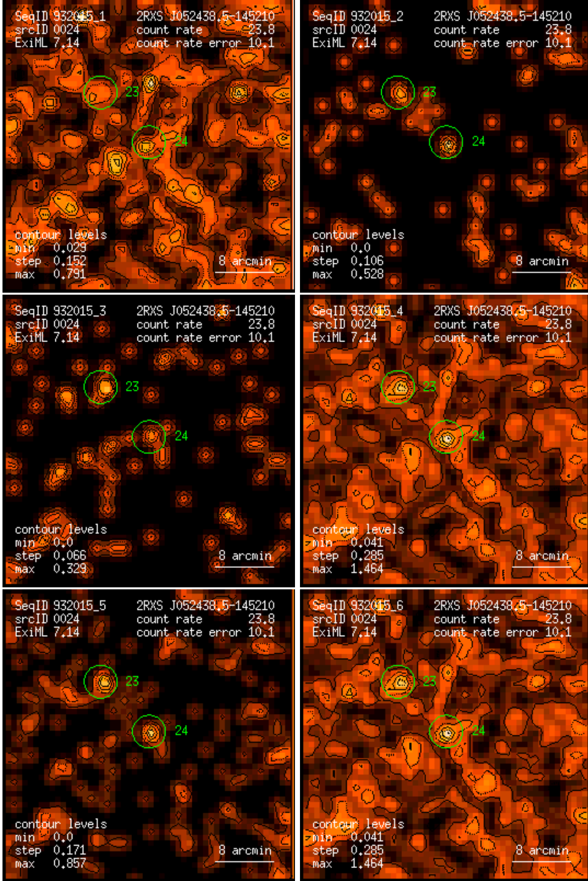
Figure 24: RASS 932015: detection 0024: band rate images, Gaussian filter: (1) PSPC channels 11 – 41, (2) 52 – 90, (3) 91 – 201, (4) 11 – 235, (5) 52 – 201, (6) 11 – 201. Broad band rates in counts/ks. Band rate contour levels in counts/ks/arcmin 2 .
