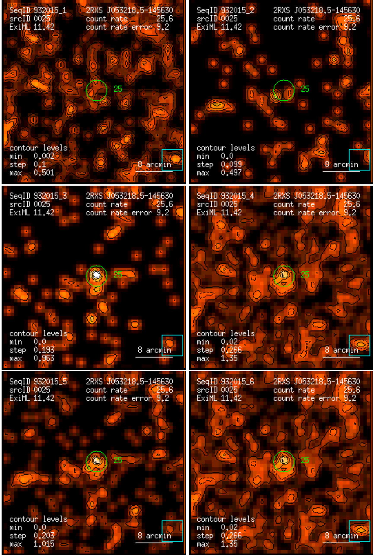
Figure 25: RASS 932015: detection 0025: band rate images, Gaussian filter: (1) PSPC channels 11 – 41, (2) 52 – 90, (3) 91 – 201, (4) 11 – 235, (5) 52 – 201, (6) 11 – 201. Broad band rates in counts/ks. Band rate contour levels in counts/ks/arcmin 2 .
