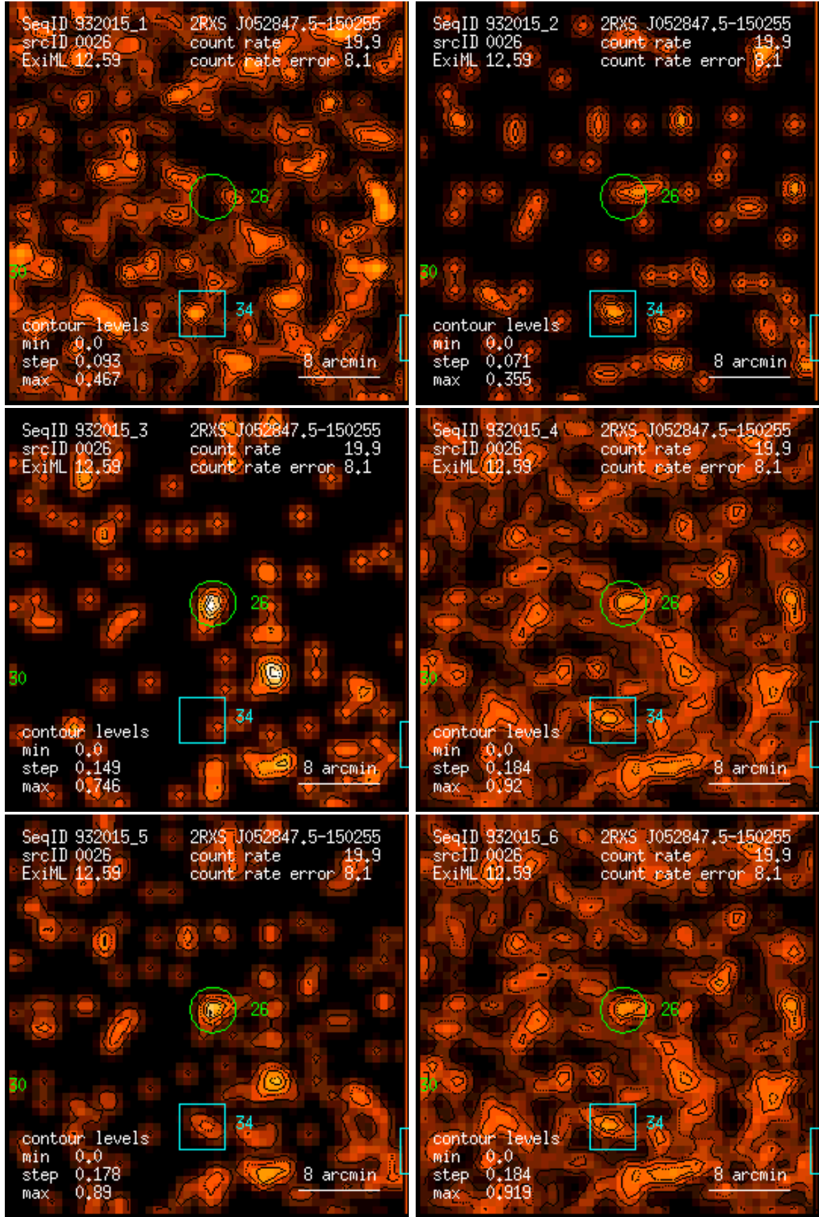
Figure 26: RASS 932015: detection 0026: band rate images, Gaussian filter: (1) PSPC channels 11 – 41, (2) 52 – 90, (3) 91 – 201, (4) 11 – 235, (5) 52 – 201, (6) 11 – 201. Broad band rates in counts/ks. Band rate contour levels in counts/ks/arcmin 2 .
