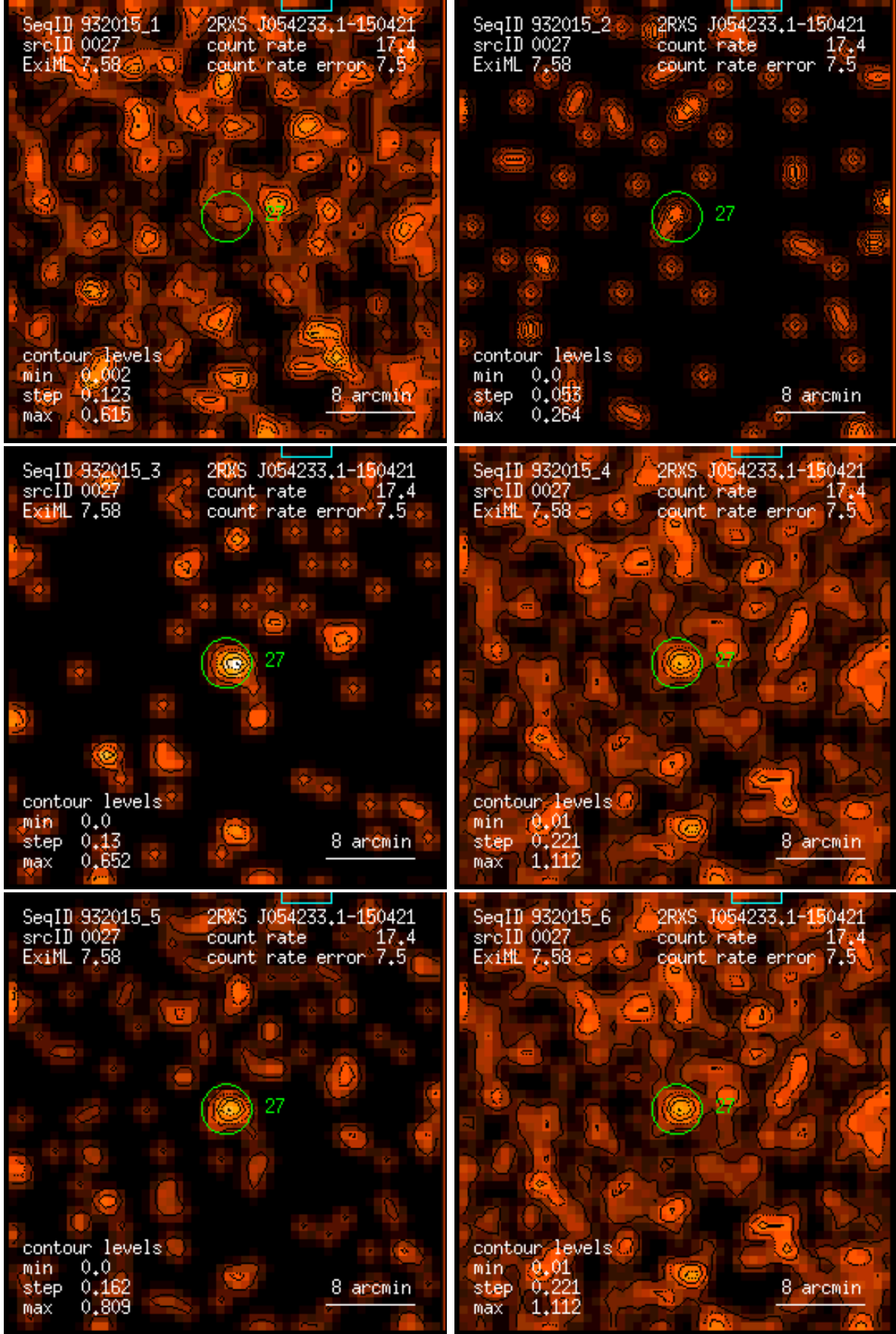
Figure 27: RASS 932015: detection 0027: band rate images, Gaussian filter: (1) PSPC channels 11 – 41, (2) 52 – 90, (3) 91 – 201, (4) 11 – 235, (5) 52 – 201, (6) 11 – 201. Broad band rates in counts/ks. Band rate contour levels in counts/ks/arcmin 2 .
