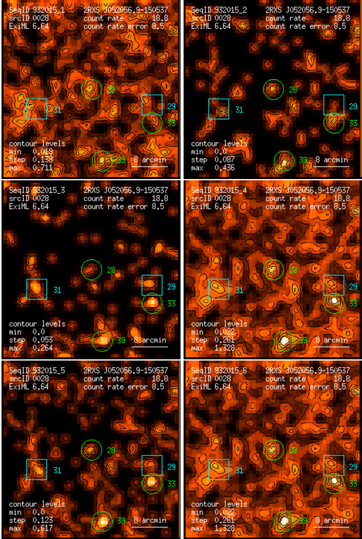
Figure 28: RASS 932015: detection 0028: band rate images, Gaussian filter: (1) PSPC channels 11 – 41, (2) 52 – 90, (3) 91 – 201, (4) 11 – 235, (5) 52 – 201, (6) 11 – 201. Broad band rates in counts/ks. Band rate contour levels in counts/ks/arcmin 2 .
