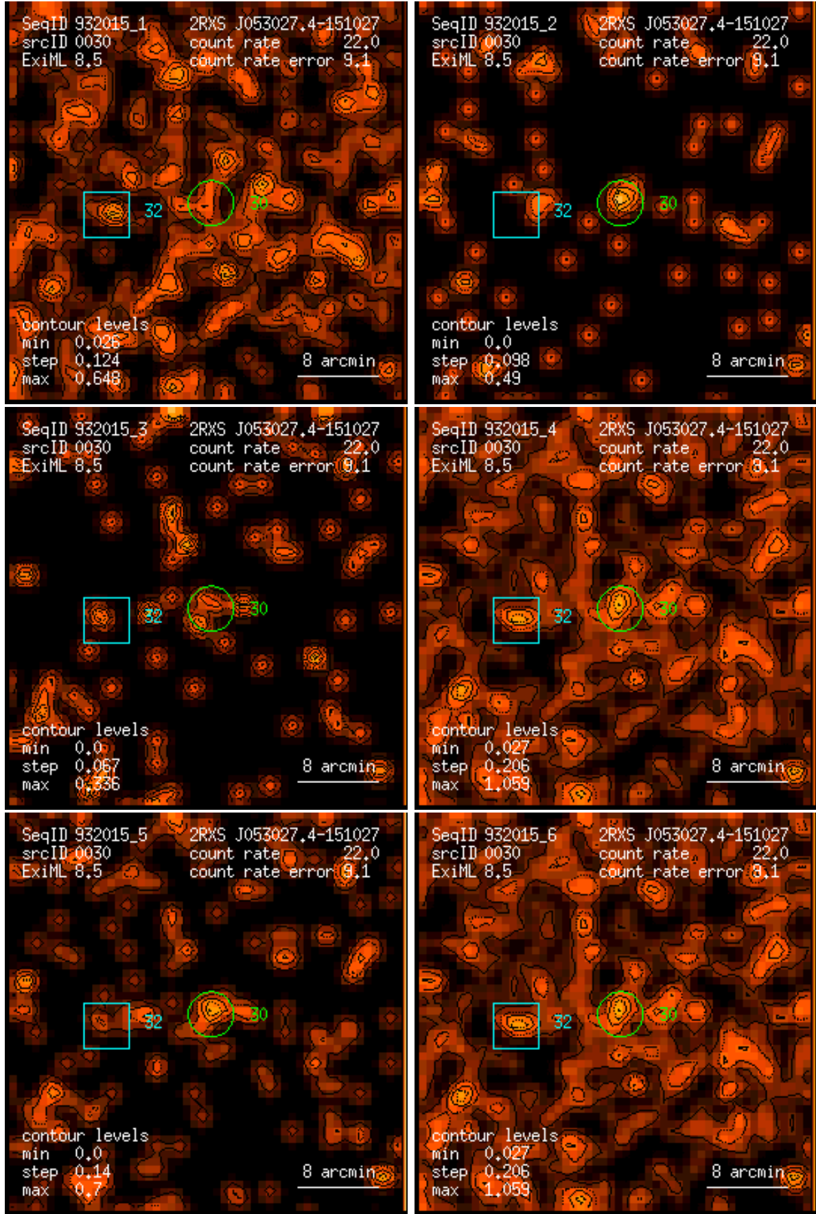
Figure 30: RASS 932015: detection 0030: band rate images, Gaussian filter: (1) PSPC channels 11 – 41, (2) 52 – 90, (3) 91 – 201, (4) 11 – 235, (5) 52 – 201, (6) 11 – 201. Broad band rates in counts/ks. Band rate contour levels in counts/ks/arcmin 2 .
