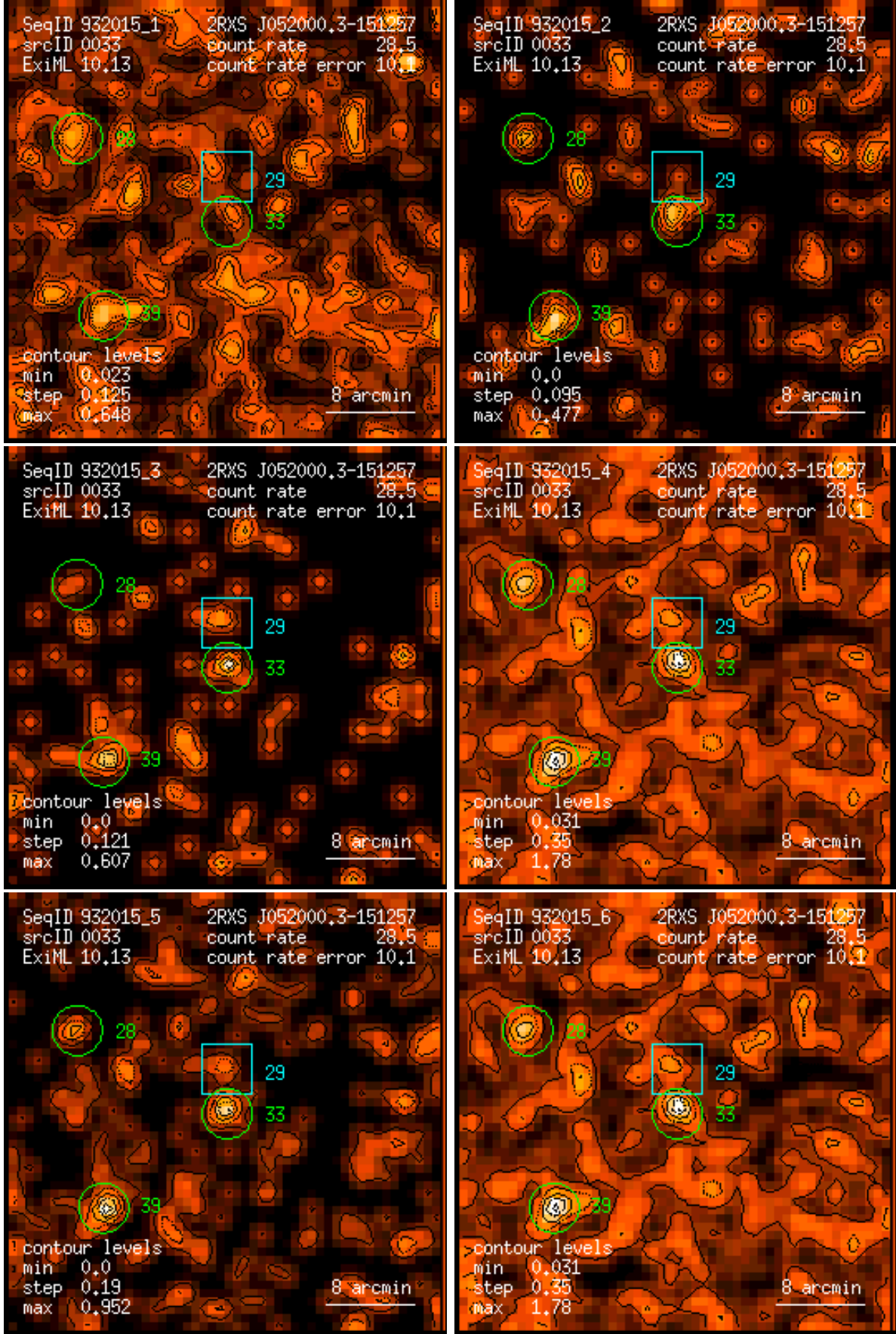
Figure 33: RASS 932015: detection 0033: band rate images, Gaussian filter: (1) PSPC channels 11 – 41, (2) 52 – 90, (3) 91 – 201, (4) 11 – 235, (5) 52 – 201, (6) 11 – 201. Broad band rates in counts/ks. Band rate contour levels in counts/ks/arcmin 2 .
