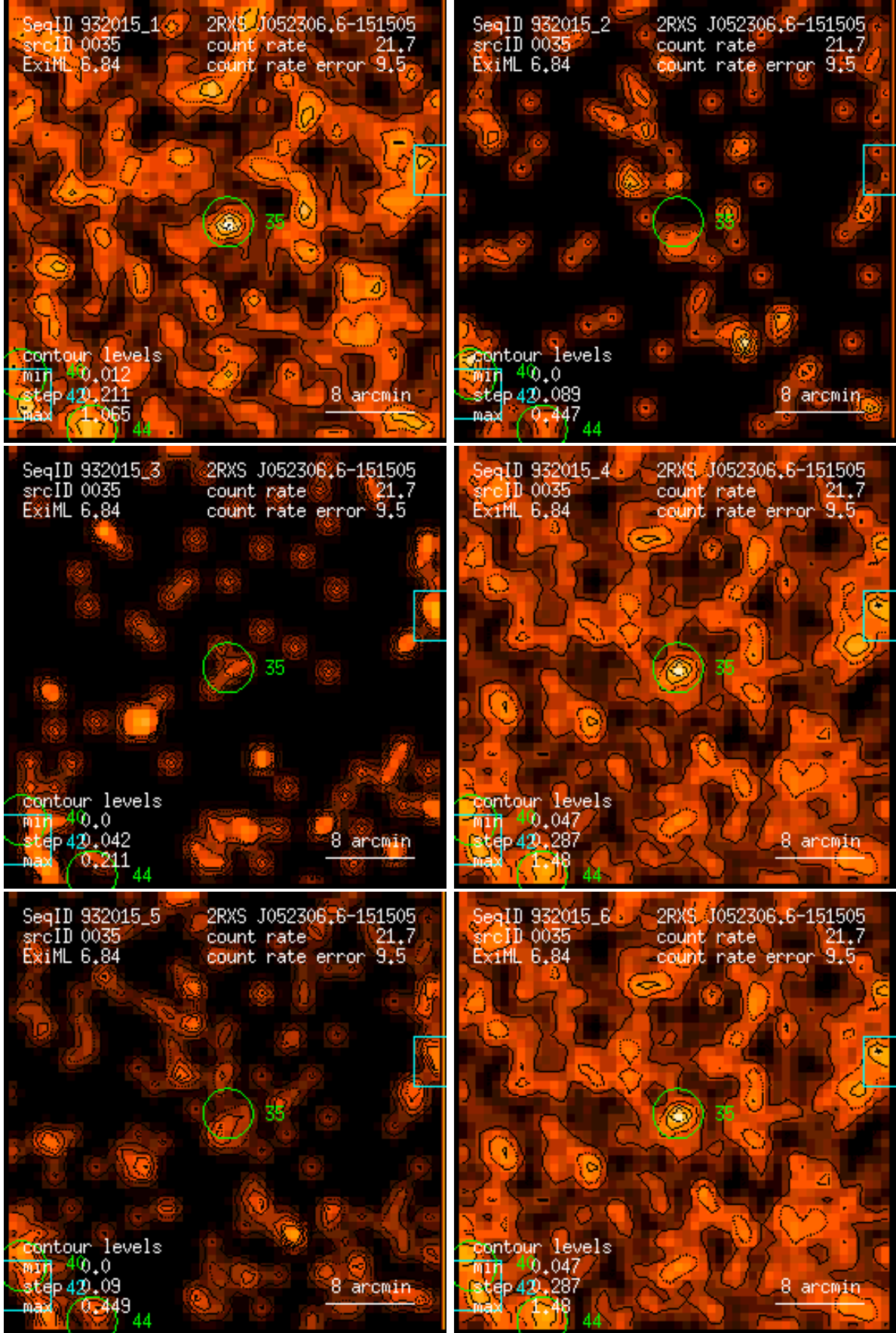
Figure 35: RASS 932015: detection 0035: band rate images, Gaussian filter: (1) PSPC channels 11 – 41, (2) 52 – 90, (3) 91 – 201, (4) 11 – 235, (5) 52 – 201, (6) 11 – 201. Broad band rates in counts/ks. Band rate contour levels in counts/ks/arcmin 2 .
