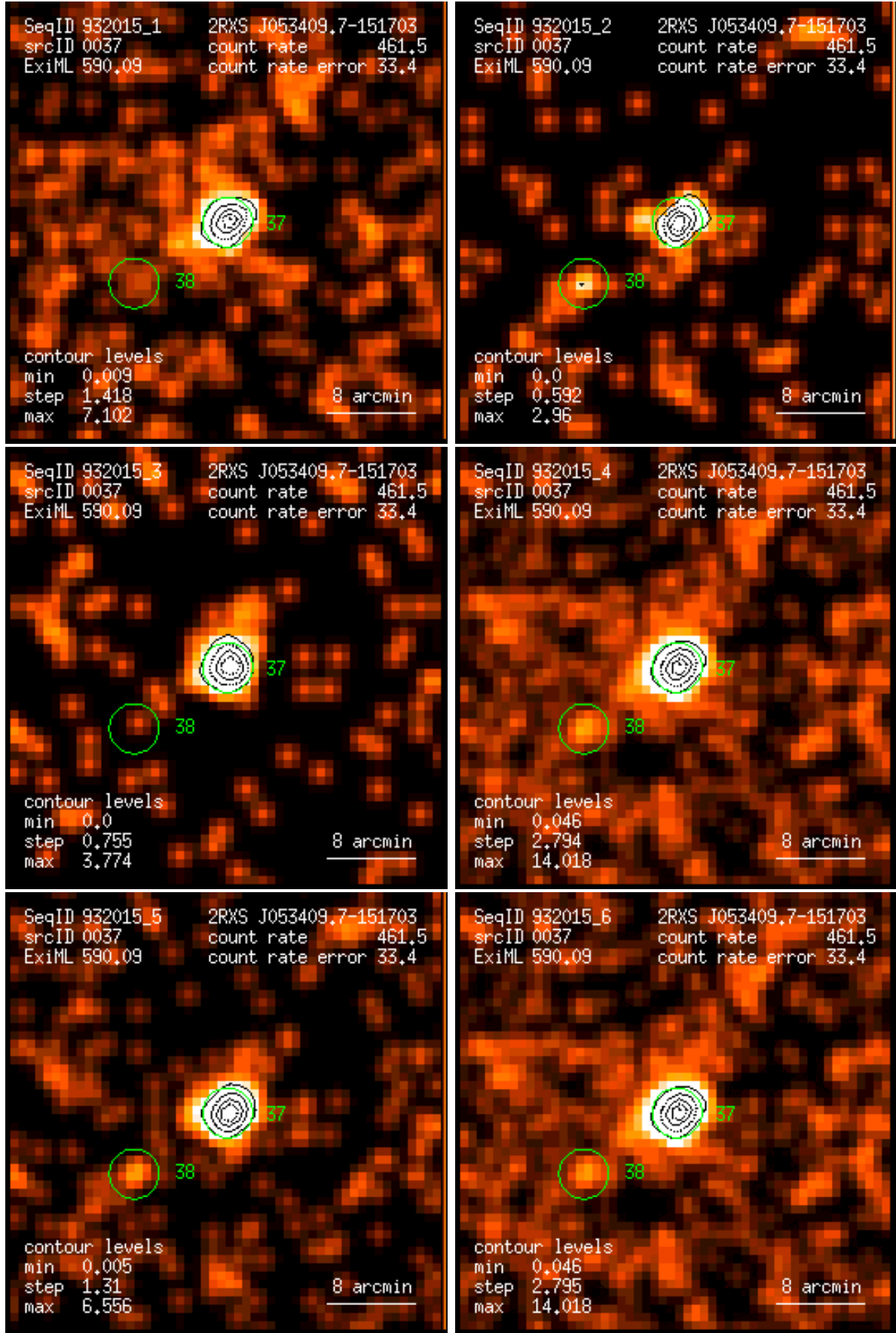
Figure 37: RASS 932015: detection 0037: band rate images, Gaussian filter: (1) PSPC channels 11 – 41, (2) 52 – 90, (3) 91 – 201, (4) 11 – 235, (5) 52 – 201, (6) 11 – 201. Broad band rates in counts/ks. Band rate contour levels in counts/ks/arcmin 2 .
