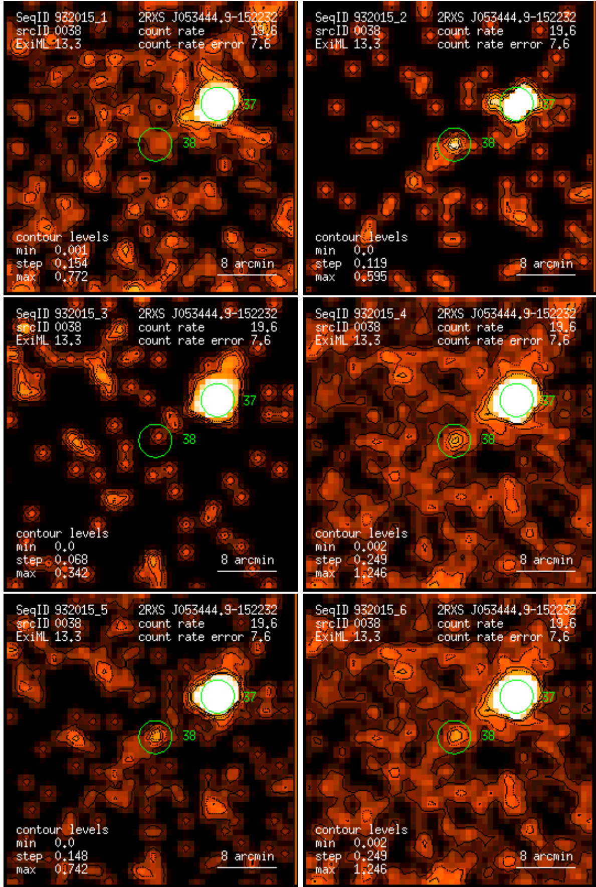
Figure 38: RASS 932015: detection 0038: band rate images, Gaussian filter: (1) PSPC channels 11 – 41, (2) 52 – 90, (3) 91 – 201, (4) 11 – 235, (5) 52 – 201, (6) 11 – 201. Broad band rates in counts/ks. Band rate contour levels in counts/ks/arcmin 2 .
