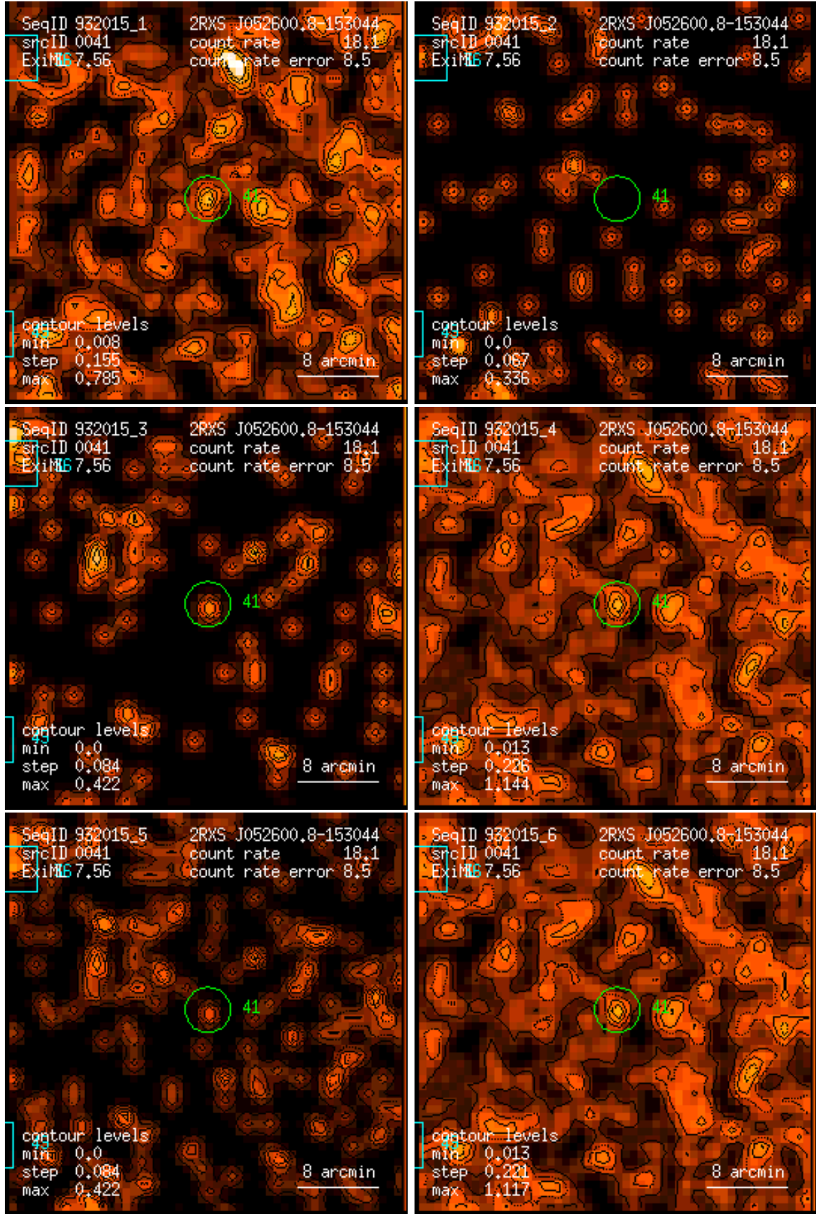
Figure 41: RASS 932015: detection 0041: band rate images, Gaussian filter: (1) PSPC channels 11 – 41, (2) 52 – 90, (3) 91 – 201, (4) 11 – 235, (5) 52 – 201, (6) 11 – 201. Broad band rates in counts/ks. Band rate contour levels in counts/ks/arcmin 2 .
