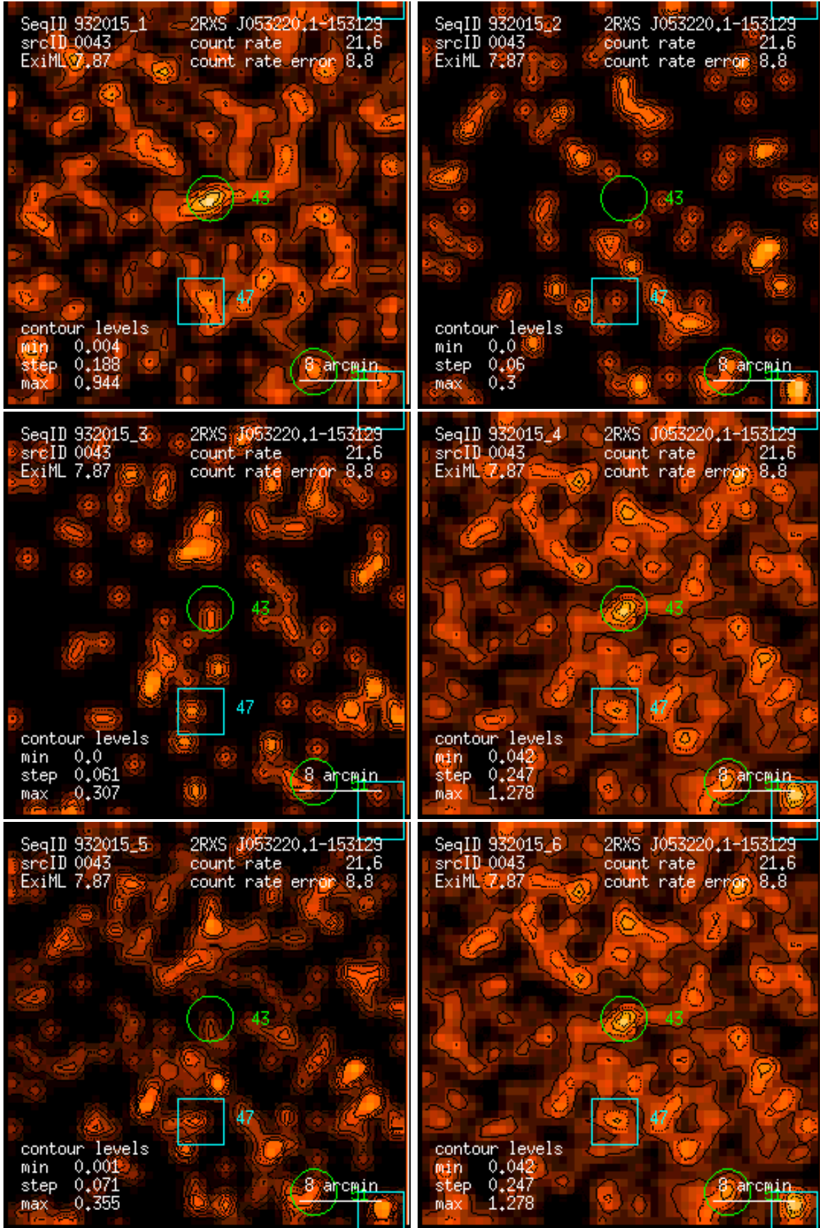
Figure 43: RASS 932015: detection 0043: band rate images, Gaussian filter: (1) PSPC channels 11 – 41, (2) 52 – 90, (3) 91 – 201, (4) 11 – 235, (5) 52 – 201, (6) 11 – 201. Broad band rates in counts/ks. Band rate contour levels in counts/ks/arcmin 2 .
