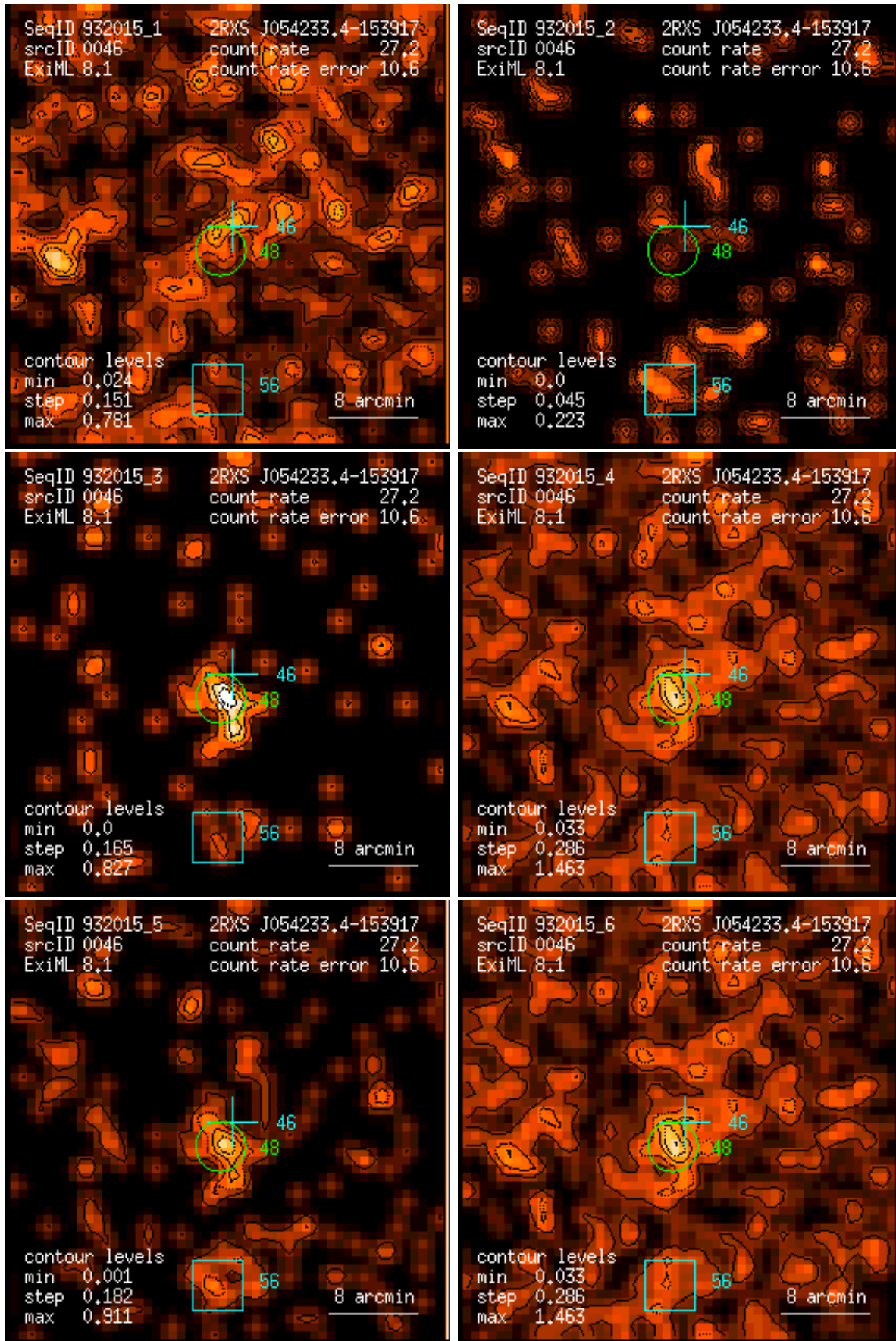
Figure 46: RASS 932015: detection 0046: band rate images, Gaussian filter: (1) PSPC channels 11 – 41, (2) 52 – 90, (3) 91 – 201, (4) 11 – 235, (5) 52 – 201, (6) 11 – 201. Broad band rates in counts/ks. Band rate contour levels in counts/ks/arcmin 2 .
