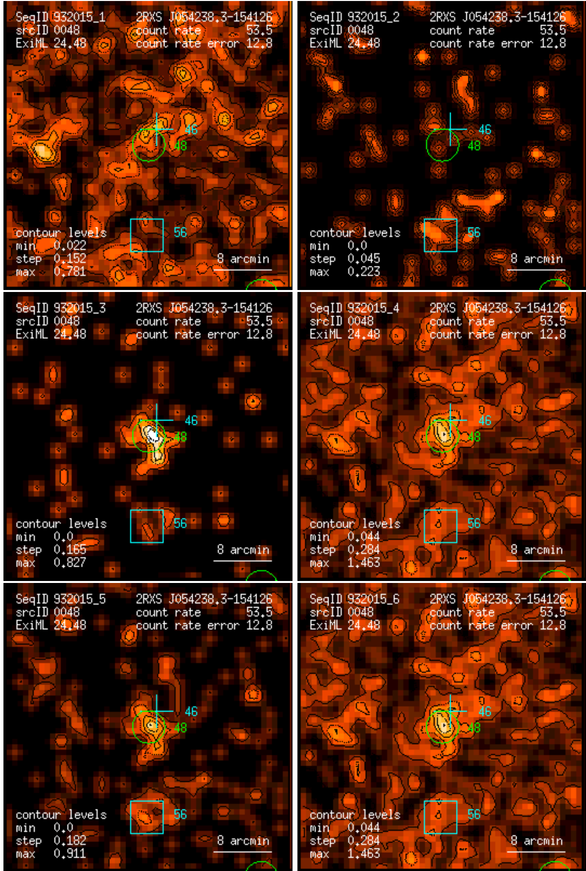
Figure 48: RASS 932015: detection 0048: band rate images, Gaussian filter: (1) PSPC channels 11 – 41, (2) 52 – 90, (3) 91 – 201, (4) 11 – 235, (5) 52 – 201, (6) 11 – 201. Broad band rates in counts/ks. Band rate contour levels in counts/ks/arcmin 2 .
