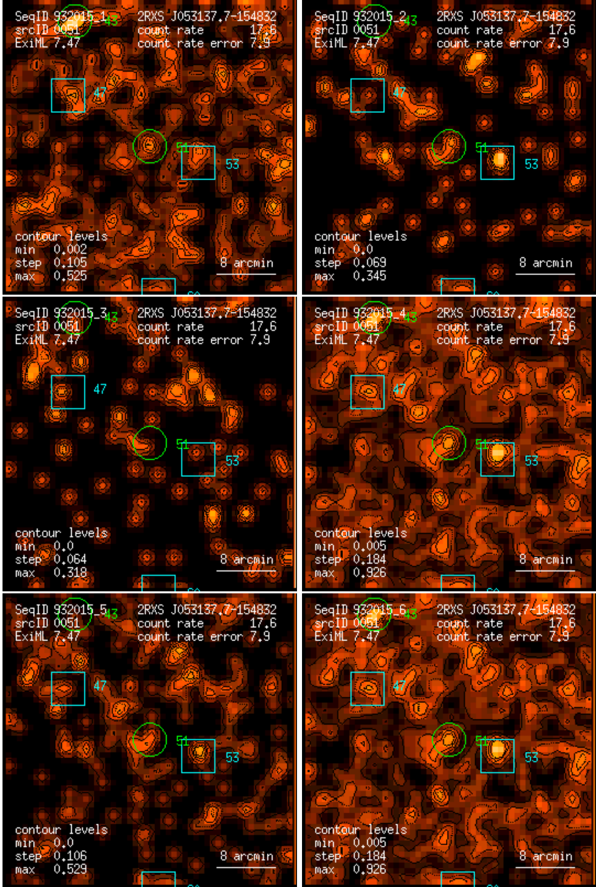
Figure 51: RASS 932015: detection 0051: band rate images, Gaussian filter: (1) PSPC channels 11 – 41, (2) 52 – 90, (3) 91 – 201, (4) 11 – 235, (5) 52 – 201, (6) 11 – 201. Broad band rates in counts/ks. Band rate contour levels in counts/ks/arcmin 2 .
